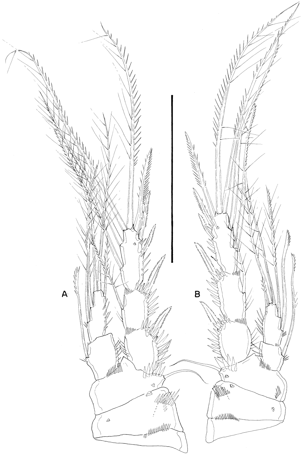
Figure 6. Mesochra ingolfssoni sp. nov., female. (A) P3; (B) P4. Scale bar: 100 µm.
