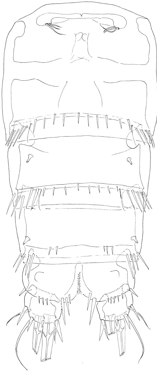
Figure 11. Mesochra snoppa sp. nov., female. Urosome, ventral, P5-bearing somite omitted. Scale bar: 100 \mu m.
