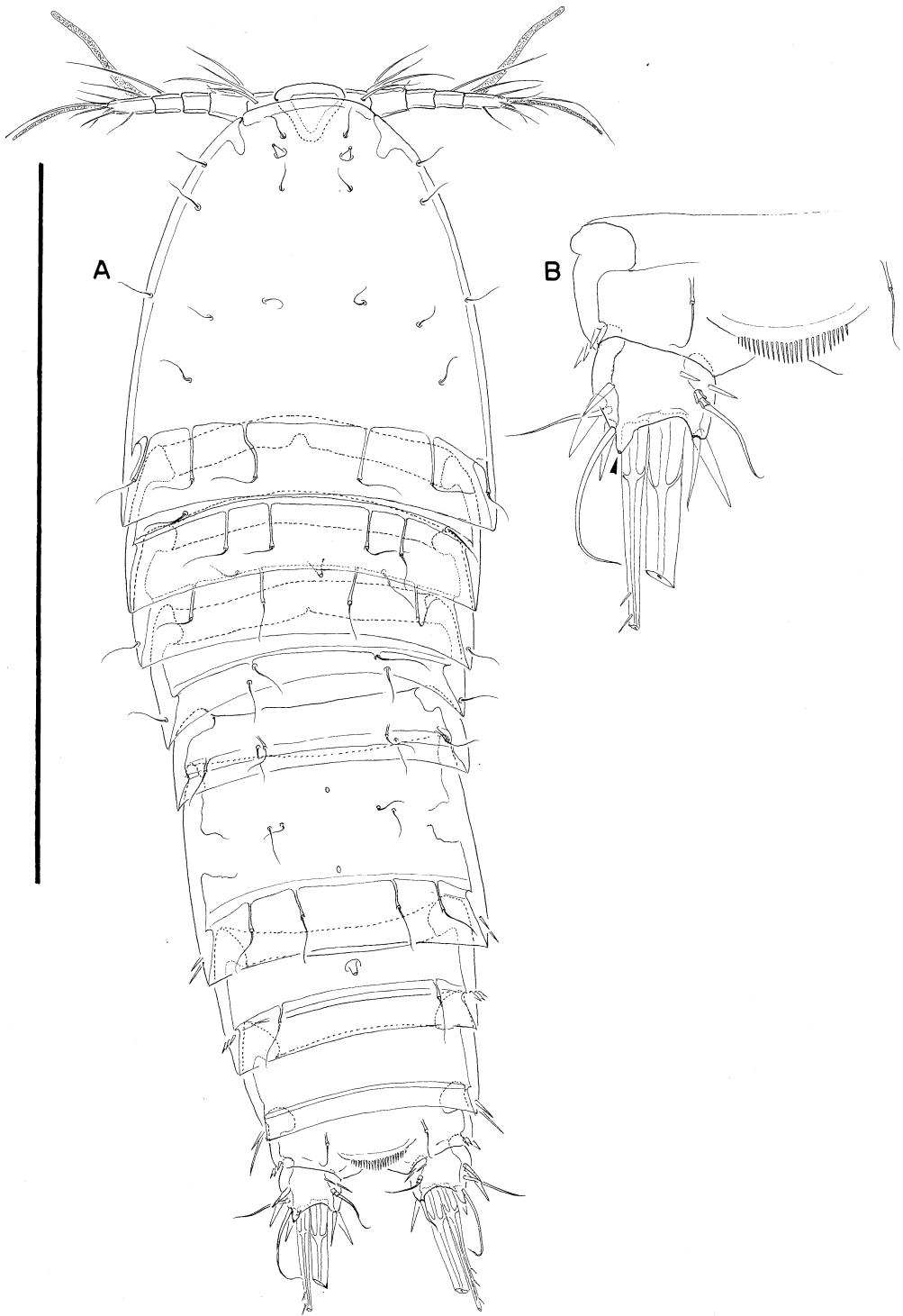
Figure 9. Mesochra snoppa sp. nov., female. (A) Habitus, dorsal; (B) anal somite and left caudal ramus, dorsal, distal outer pore arrowed. Scale bar: 200 \mu m (A); 100 \mu m (B).
