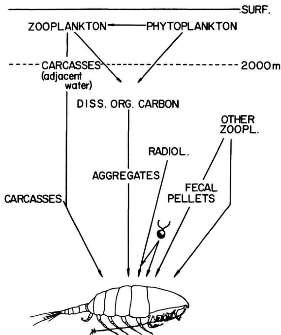
FIGURE 4.—Sources of food for deep-sea copepods. The flagellate represents unicellular organisms other than Radiolaria.
