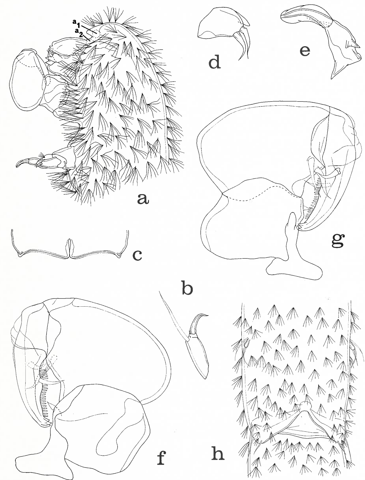
Fig. 6. Xarifia villosa n. sp., male. a, cephalothorax, lateral ( a_1 = position of first antenna, a_2 = position of second antenna) (scale I); b, fourth segment of second antenna, ventral (K); c, posterior edge of labrum, ventral (F); d, first maxilla, inner (K); e, second segment of second maxilla, posteroventral (K); f, maxilliped, outer (F); g, maxilliped, inner (F); h, leg 5 and 6, ventral (I).
