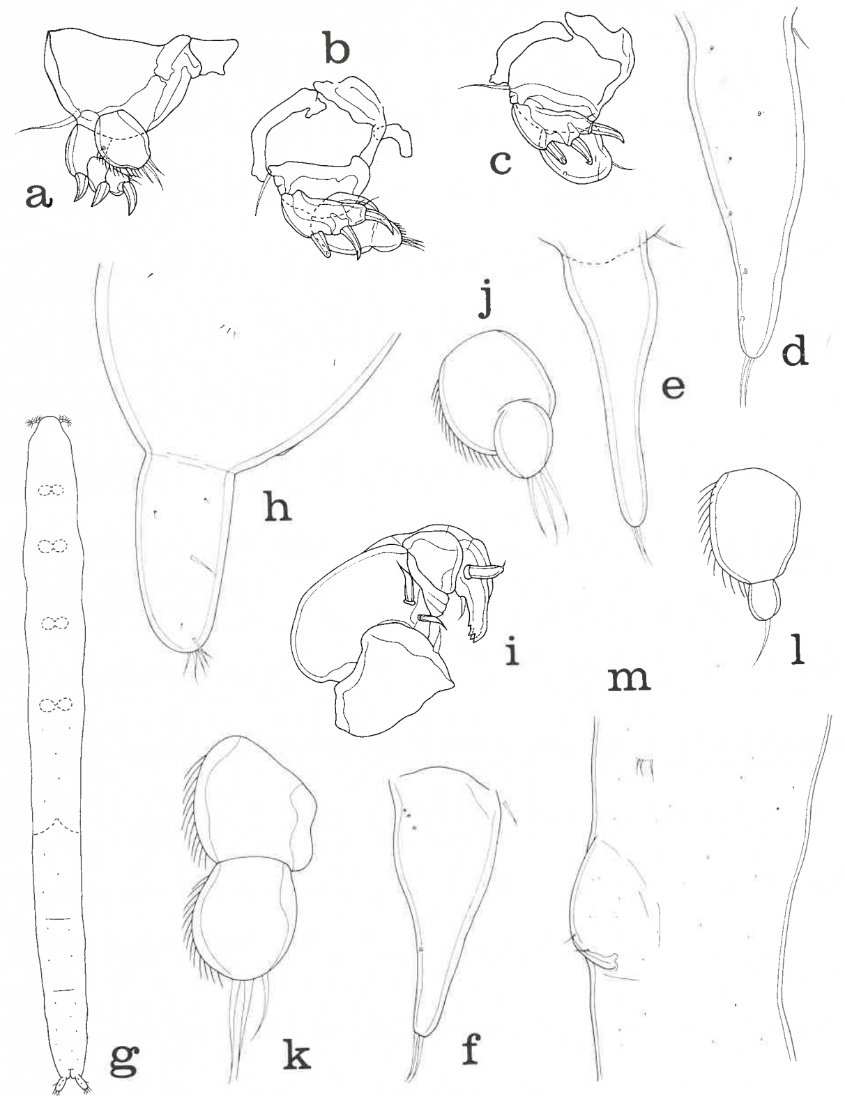
Fig. 20. Xarifia mucronata n. sp. Female. a, leg 1 and intercoxal plate, anterior (scale F); b, leg 2 and intercoxal plate, posterior (F); c, leg 3, posterior (F); d, leg 5, lateral (F); e, leg 5, lateral (F); f, leg 5, lateral (F). Male. g, dorsal (M); h, caudal ramus, lateral (F); i, maxilliped, inner (F); j, endopod of leg 1, posterior (N); k, endopod of leg 2, posterior (N); l, endopod of leg 4, posterior (N); m, leg 5 and leg 6, lateral (I).
