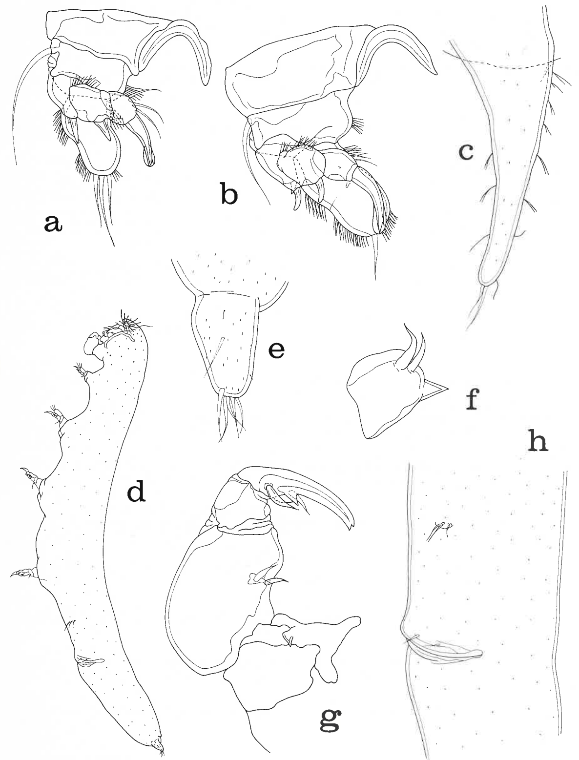
Fig. 47. Xarifia tumorisa Misaki, 1978. Female. a, leg 1 and intercoxal plate, posterior (scale F); b, leg 3 and intercoxal plate, posterior (F); c, leg 5, lateral (D). Male. d, lateral (L); e, caudal ramus, lateral (F); f, first maxilla, antero-inner (N); g, maxilliped, inner (F); h, leg 5 and leg 6, lateral (I).
