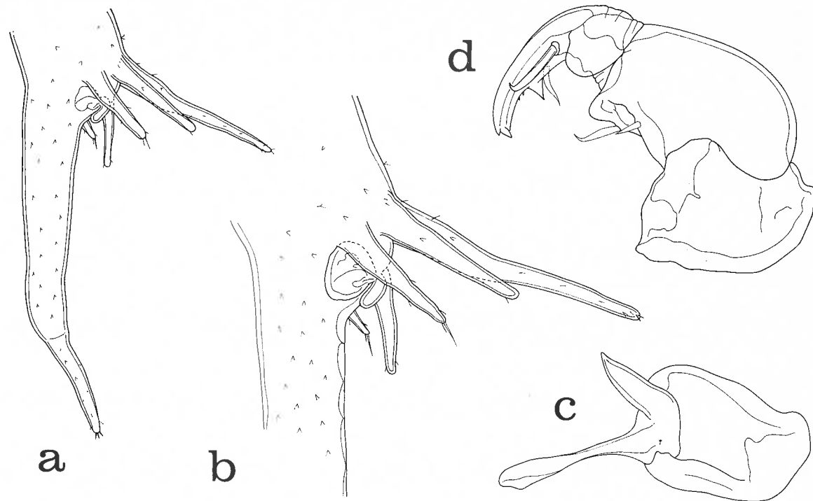
Fig. 45. Xarifia sabiuraensis Misaki, 1978, female from Acropora affinis . a, urosome, lateral (scale J); b, genital area, lateral (C). Male. c, second maxilla, posteroventral (N); d, maxilliped, inner (F).
