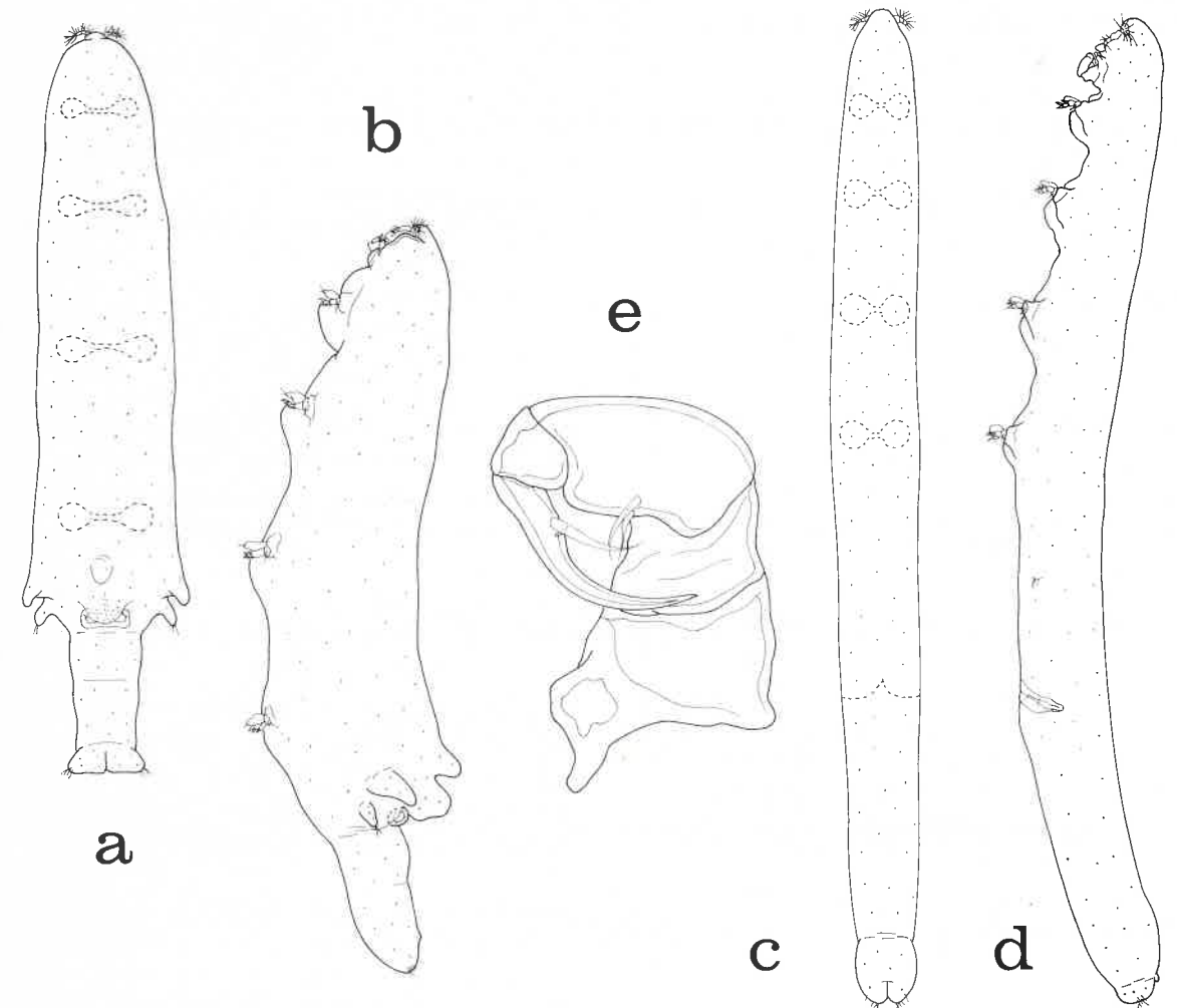
Fig. 48. Xarifia gerlachi Humes, 1962. Female. a, dorsal (scale H); b, lateral (H). Male c, dorsal (B); d, lateral (B); e, maxilliped, inner (K).
