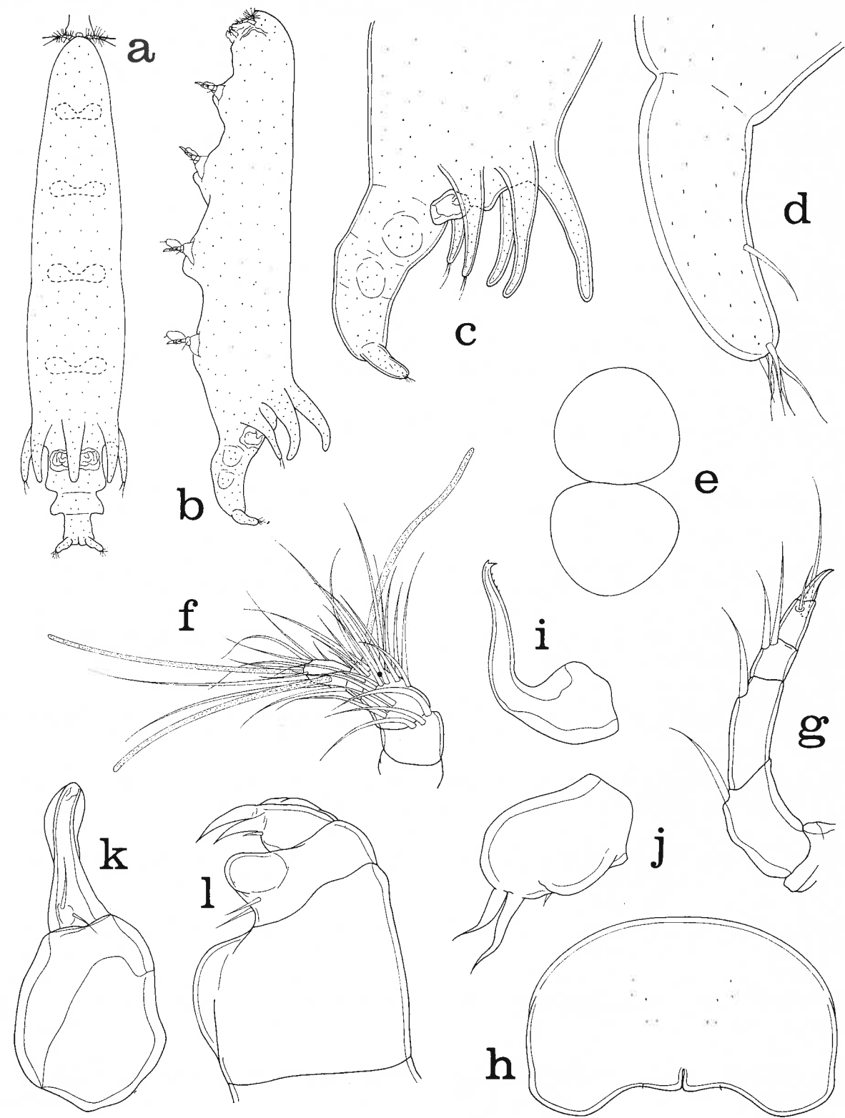
Fig. 46. Xarifia tumorisa Misaki, 1978, female. a, dorsal (scale M); b, lateral (M); c, urosome, lateral (J); d, caudal ramus, lateral (F); e, egg sac, lateral (J); f, first antenna, with dot indicating position of aesthete added in male, anterodorsal (F); g, second antenna, dorso-inner (K); h, labrum, ventral (K); i, mandible, ventral (N); j, first maxilla, anteroventral (N); k, second maxilla, antero-inner (N); l, maxilliped, anterior (N).
