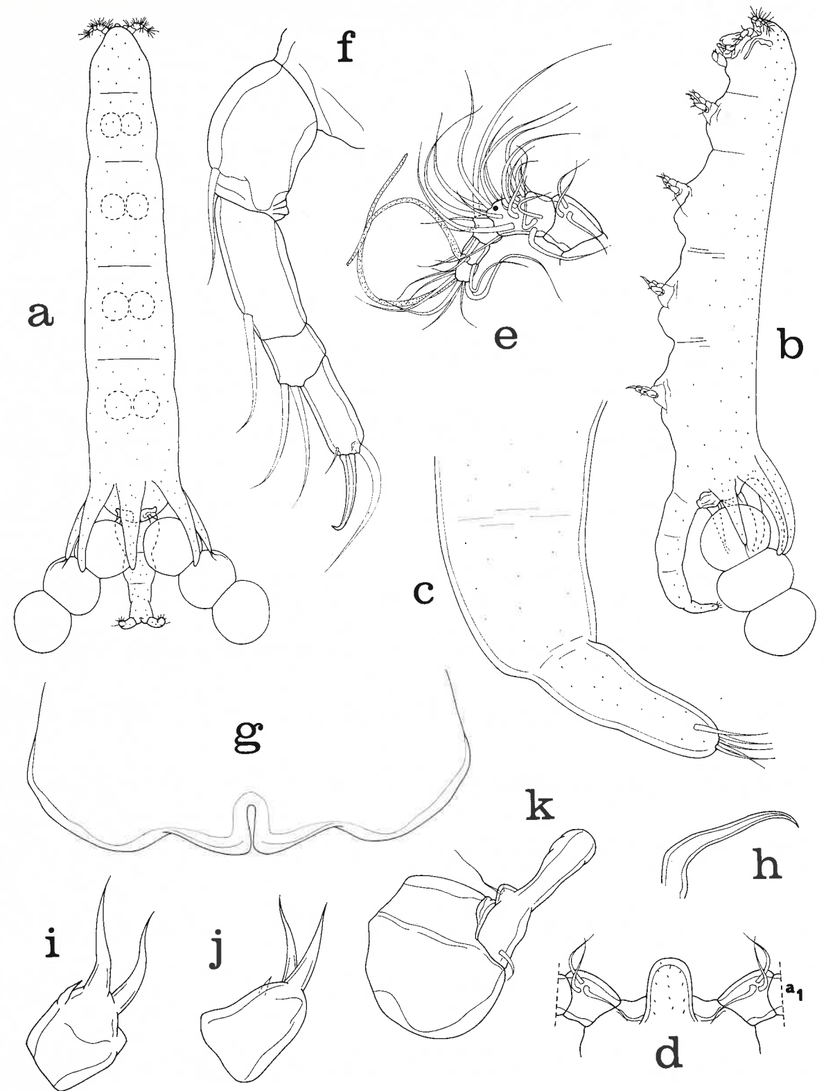
Fig. 15. Xarifia ablusa n. sp., female. a, dorsal (scale B); b, lateral (B); c, caudal ramus, lateral (F); d, rostrum (a 1 = position of first antenna), dorsal (F); e, first antenna, with dot indicating position of aesthete added in male, anterodorsal (F); f, second antenna, dorsal (N); g, labrum, ventral (N); h, mandible, ventral (N); i, first maxilla, ventro-outer (N); j, first maxilla, dorsal (N); k, second maxilla, antero-outer (N).
