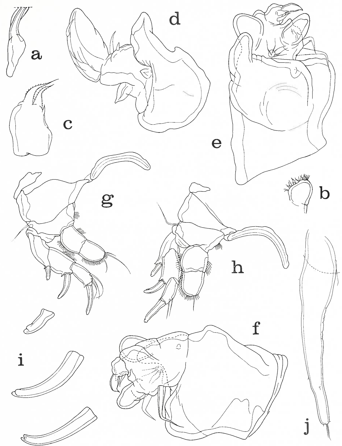
Fig. 31. Xarifia radians n. sp., female. a, mandible, broken tip, ventral (scale E); b, paragnath, outer (E); c, first maxilla, anteroventral (E); d, second maxilla, antero-inner (F); e, maxilliped, inner (F); f, maxilliped, postero-outer (F); g, leg 1 and intercoxal plate, anterior (I); h, leg 3 and intercoxal plate, anterior (I); i, spines of exopod of leg 2, posterior (F); j, leg 5, lateral (G).
