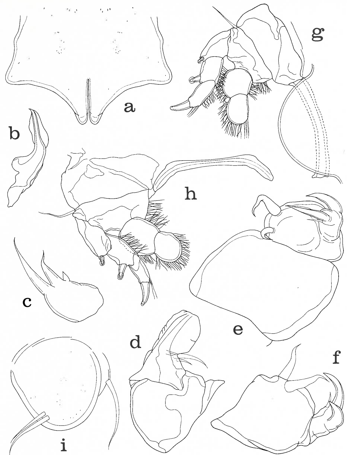
Fig. 28. Xarifia mediolobata n. sp., female. a, labrum, ventral (scale E); b, mandible, ventral (F); c, first maxilla, anterioventral (F); d, second maxilla, postero-outer (F); e, maxilliped, antero-inner (F); f, distal portion of maxilliped, anterior (F); g, leg 1 and intercoxal plate, posterior (I); h, leg 3 and intercoxal plate, posterior (I); i, leg 5, lateral (E).
