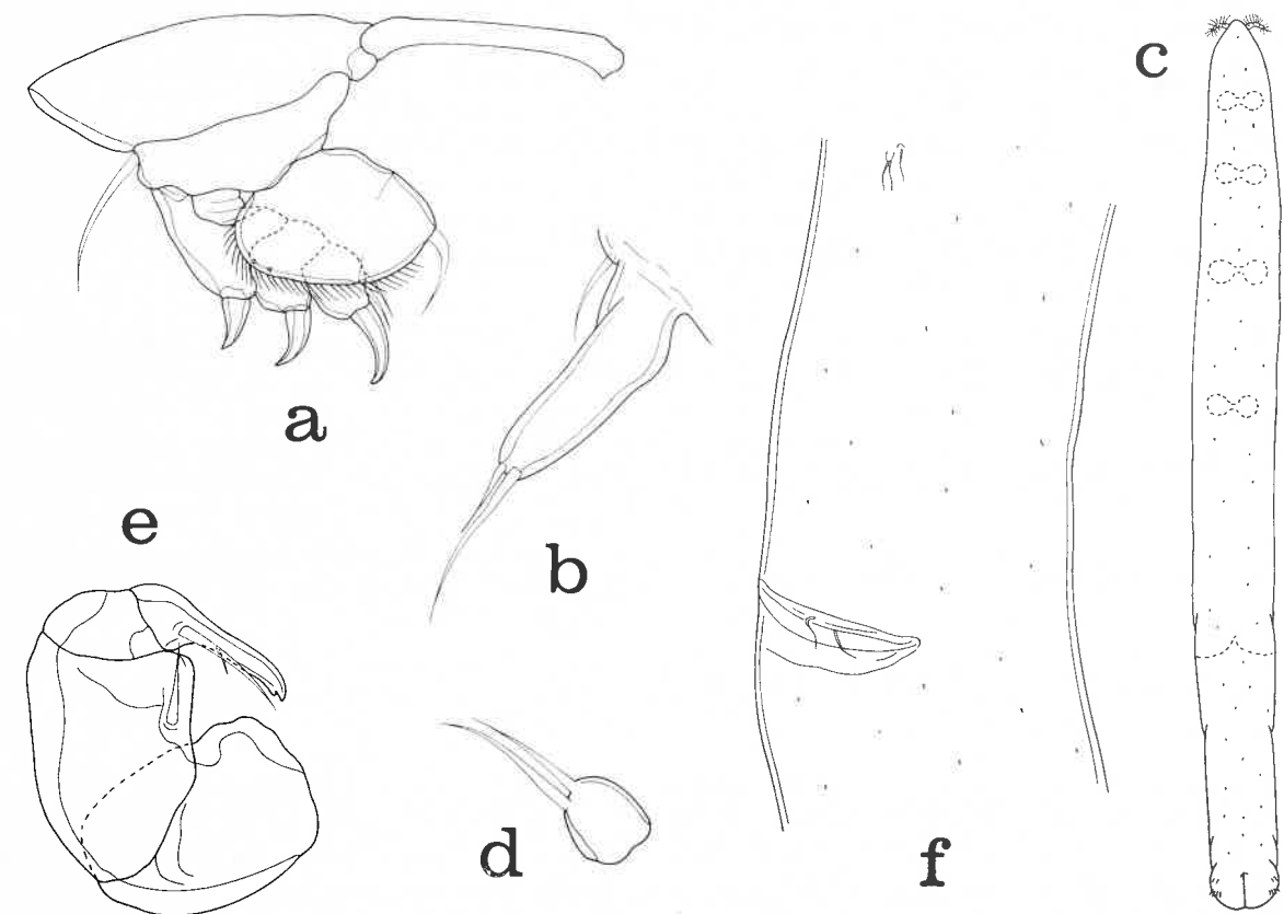
Fig. 14. Xarifia trituberata n. sp. Female. a, leg 3 and intercoxal plate, anterior (scale F); b, leg 5, ventro-lateral (F). Male. c, dorsal (M); d, first maxilla, anterior (N); e, maxilliped, medial (N); f, leg 5 and leg 6, lateral (I).
