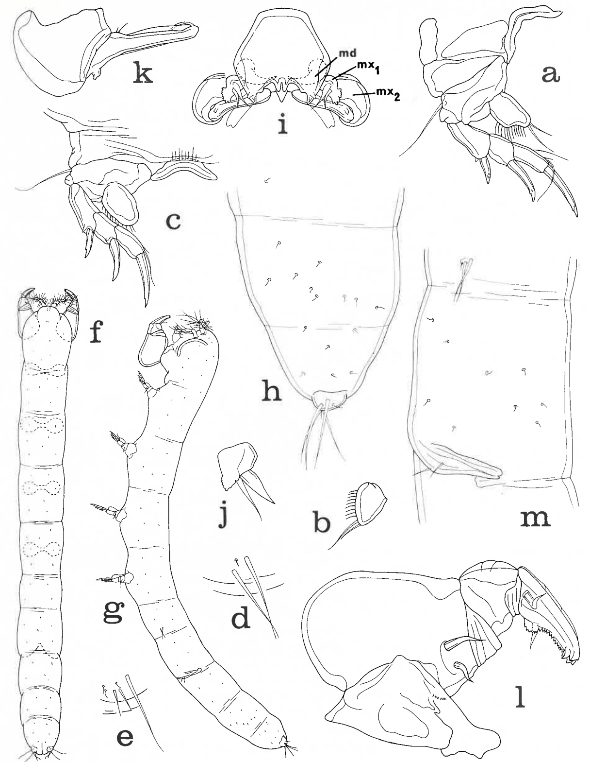
Fig. 36. Xarifia syntoma n. sp., Female. a, leg 2 and intercoxal plate, posterior (scale F); b, endopod of leg 2, posterior (F); c, leg 3 and intercoxal plate, anterior (F); d, leg 5, lateral (F); e, leg 5, aberrant specimen, lateral (F). Male. f, dorsal (J); g, lateral (J); h, posterior part of urosome and caudal ramus, lateral (F); i, labrum, with mandibles (md), first maxillae (mx 1 ), and second maxillae (mx 2 ) in position, ventral (F); j, first maxilla, postero-outer (N); k, second maxilla, antero-inner (N); l, maxilliped, inner (F); m, leg 5 and leg 6, lateral (E).
