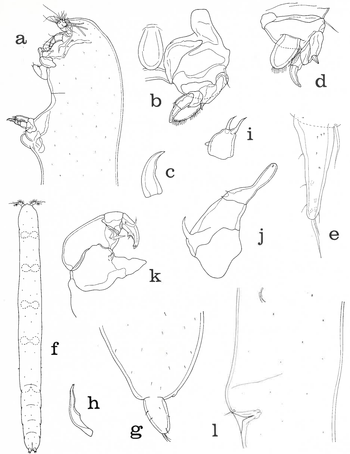
Fig. 42. Xarifia sabiuraensis Misaki, 1978. Female. a, cephalosome and first pedigerous segment, lateral (scale 1); b, leg 1, intercoxal plate, and median bulbous protrusion, posterior (F); c, spine of third segment of exopod of leg 1, posterior (N); d, leg 2, anterior (F); e, leg 5, lateral (F). Male. f, dorsal (B); g, caudal ramus, lateral (F); h, mandible, ventral (N); i, first maxilla, anteroventral (N); j, second maxilla, posteroventral (N); k, maxilliped, inner (F); l, leg 5 and leg 6, lateral (E).
