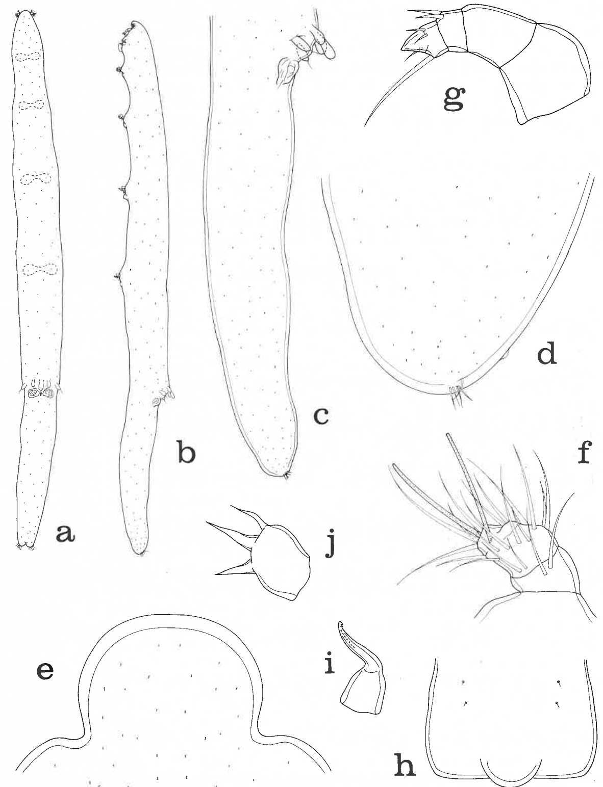
Fig. 21. Xarifia guttulifera n. sp., female. a, dorsal (scale H); b, lateral (H); c, urosome, lateral (J); d, caudal ramus, lateral (F); e, rostrum, dorsal (N); f, first antenna, anterodorsal (N); g, second antenna, dorsal (N); h, labrum, ventral (K); i, mandible, inner (N); j, first maxilla, posterodorsal (N).
