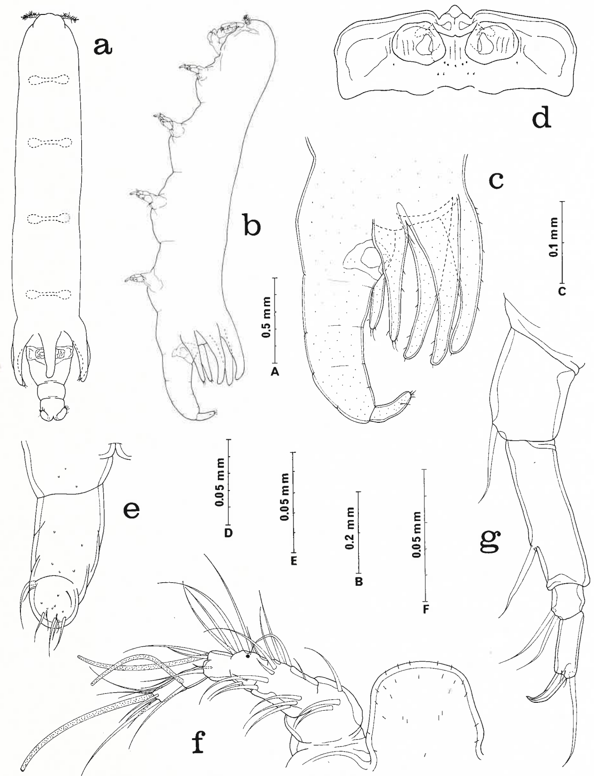
Fig. 1. Xarifia echinopora n. sp., female. a, dorsal (scale A); b, lateral (A); c, urosome, lateral (B); d, genital area, dorsal (C); e, caudal ramus, dorsal (D); f, rostrum and first antenna, with dot indicating position of aesthete added in male, anterodorsal (E); g, second antenna, dorsal (F).
