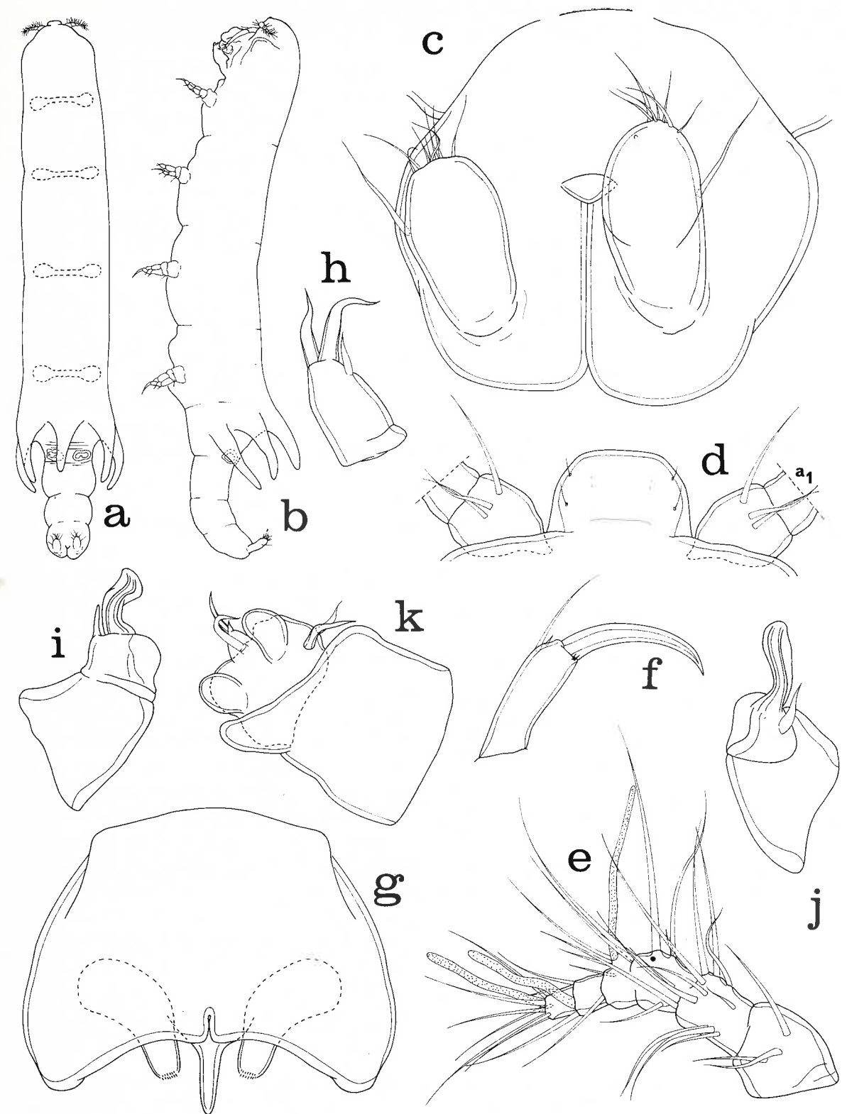
Fig. 50. Xarifia dispar Humes, 1962, female. a, dorsal (scale M); b, lateral (M); c, anal segment, dorsal, and caudal rami, ventral (F); d, rostrum (a 1 = first antenna), dorsal (F); e, first antenna, with dot indicating position of aesthete added in male, anterodorsal (F); f, last segment of second antenna, dorsal (K); g, labrum, paragnaths and medial process (labium?), ventral (F); h, first maxilla, antero-ventral (F); i, second maxillae postero-inner (F); j, second maxilla, antero-inner (F); k, maxilliped, inner (F).
