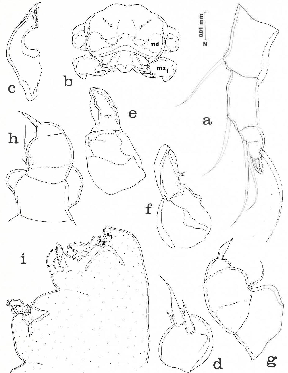
Fig. 8. Xarifia pectinea n. sp., female. a, second antenna, dorsal (scale N); b, labrum, mandible (md), and first maxilla (mx 1 ), ventral (F); c, mandible, ventral (N); d, first maxilla, posteroventral (N); e, second maxilla, anteroventral (K); f, second maxilla, postero-outer (K); g, maxilliped, inner (K); h, maxilliped, outer (K); i, cephalothorax (a 1 = position of first antenna, a 2 = position of second antenna), lateral (C).
