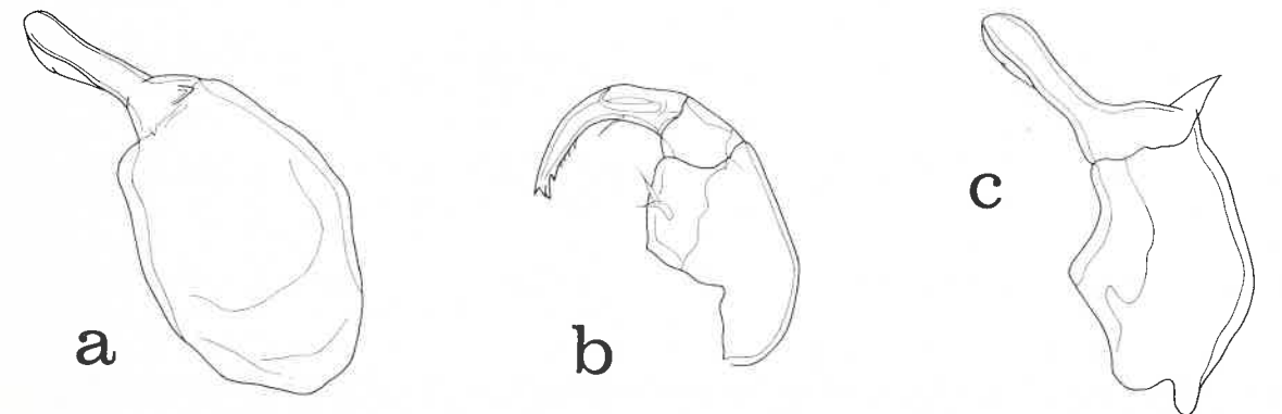
Fig. 49. Xarifia infrequens Humes, 1962, male. a, second maxilla, posteroventral (scale N); b, maxilliped (first segment not shown), inner (F). Xarifia tenuis Humes, 1962, male. c, second maxilla, antero-inner (N).
