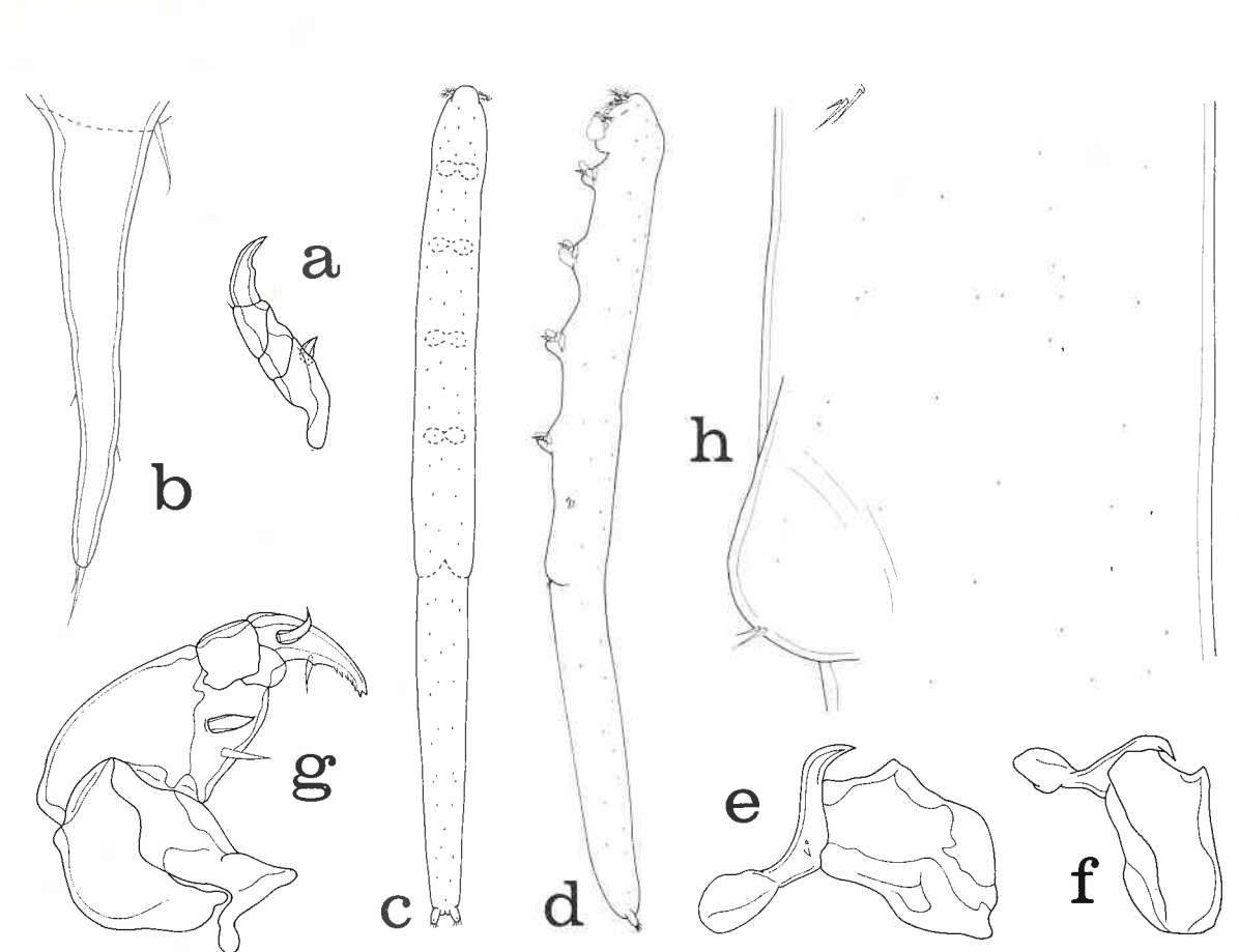
Fig. 24. Xarifia rosariae n. sp. Female. a, exopod of leg 2, posterior (scale F); b, leg 5, lateral (E). Male. c, dorsal (M); d, lateral (M); e, second maxilla, outer (K); f, second maxilla, inner (K); g, maxilliped, inner (F); h, leg 5 and leg 6, lateral (E).
