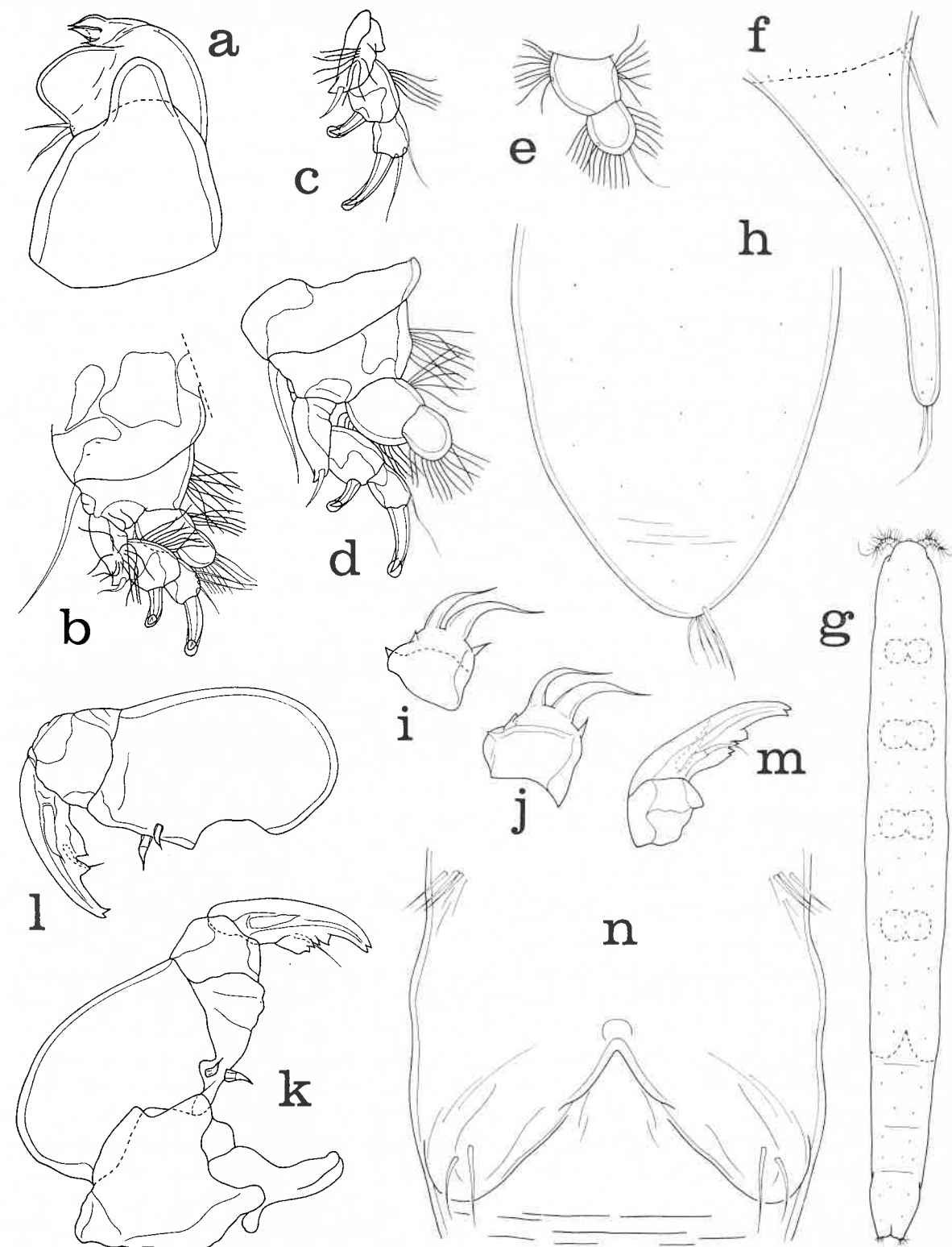
Fig. 16. Xarifia ablusa n. sp. Female. a, maxilliped, outer (scale N); b, leg 1, posterior (F); c, exopod of leg 2, posterior (F); d, leg 3, posterior (F); e, endopod of leg 4, anterior (F); f, leg 5, lateral (E). Male. g, dorsal (B); h, caudal ramus, lateral (F); i, first maxilla, inner (N); j, first maxilla, outer (N); k, maxilliped, inner (F); l, distal portion of maxilliped, inner (F); m, third segment and claw of maxilliped, outer (F); n, leg 5 and leg 6, ventral (E).
