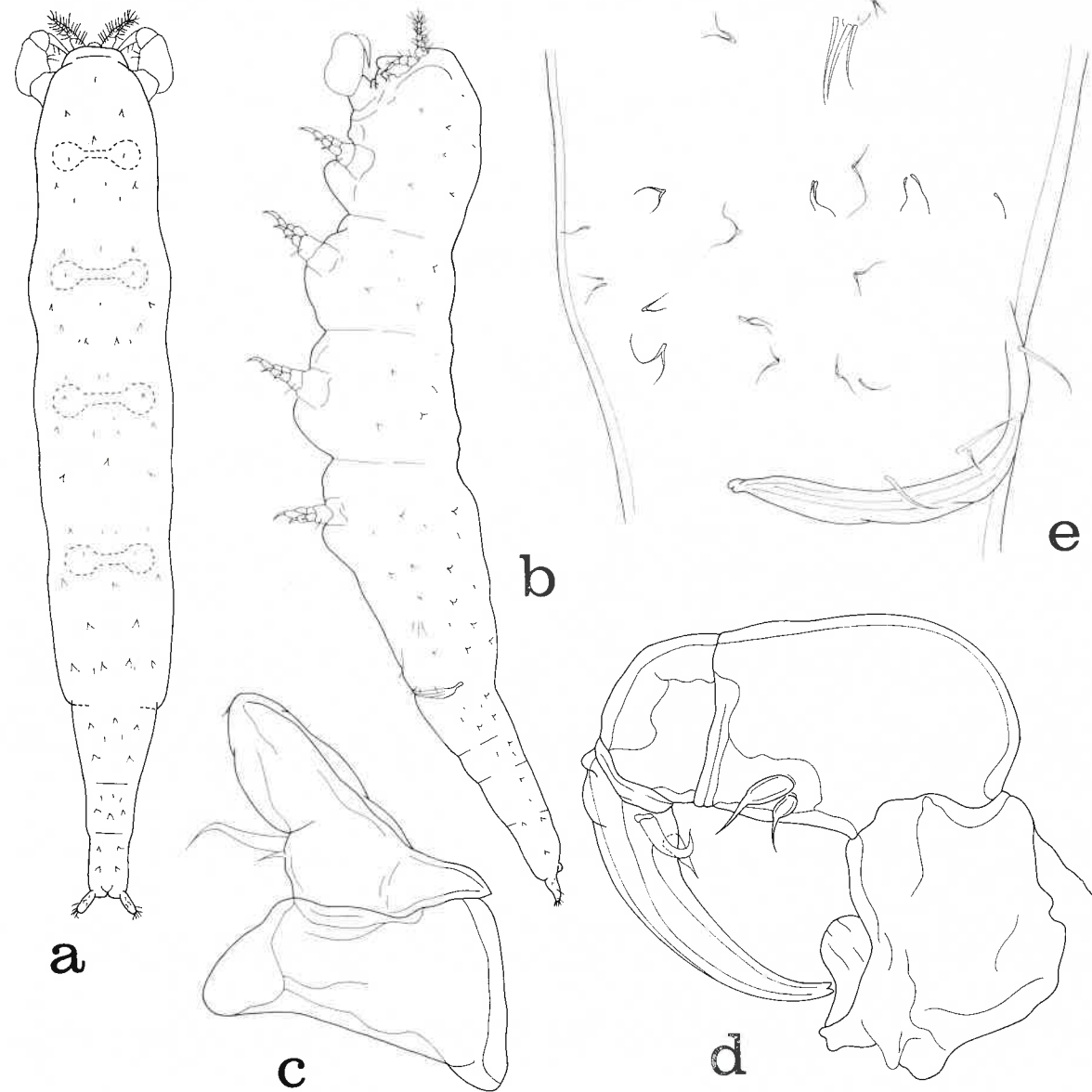
Fig. 29. Xarifia mediolobata n. sp., male. a, dorsal (scale A); b, lateral (A); c, second maxilla, postero-outer (F); d, maxilliped, inner (I); e, leg 5 and leg 6, lateral (C).
