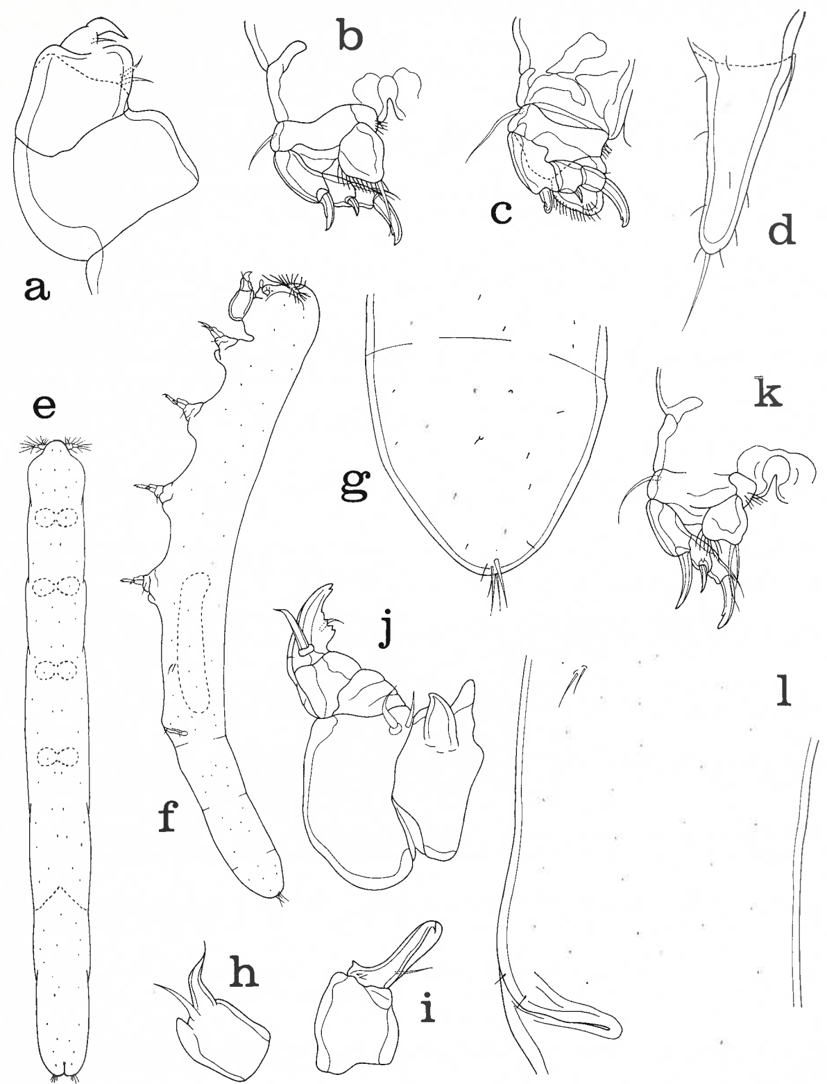
Fig. 34. Xarifia heteromeles n. sp. Female. a, maxilliped, outer (scale N); b, leg 1 and intercoxal plate, anterior (F); c, leg 3, anterior (F); d, leg 5, lateral (F). Male. e, dorsal (B); f, lateral (B); g, caudal ramus, lateral (E); h, first maxilla, ventral (N); i, second maxilla, outer (K); j, maxilliped, inner (F); k, leg 1 and intercoxal plate, anterior (F); l, leg 5 and leg 6, lateral (E).
