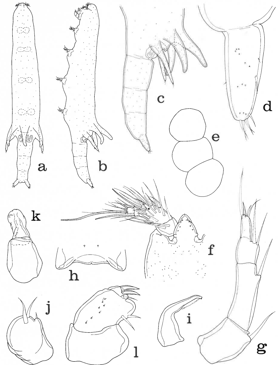
Fig. 25. Xarifia fastigiata n. sp., female. a, dorsal (scale M); b, lateral (M); c, urosome, lateral (F); d, caudal ramus, lateral (F); e, egg sac, lateral (J); f, rostrum and first antenna, with dot indicating position of aesthete added in male, dorsal (F); g, second antenna, dorsal (N); h, labrum, posteroventral (F); i, mandible, ventral (N); j, first maxilla, posteroventral (N); k, second maxilla, inner (F); l, maxilliped, inner (K).
