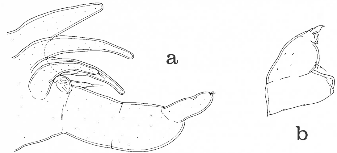
Fig. 10. Xarifia pectinea n. sp. (from Acropora patula ), female. a, urosome, lateral (scale J); b, maxilliped, inner (F).
