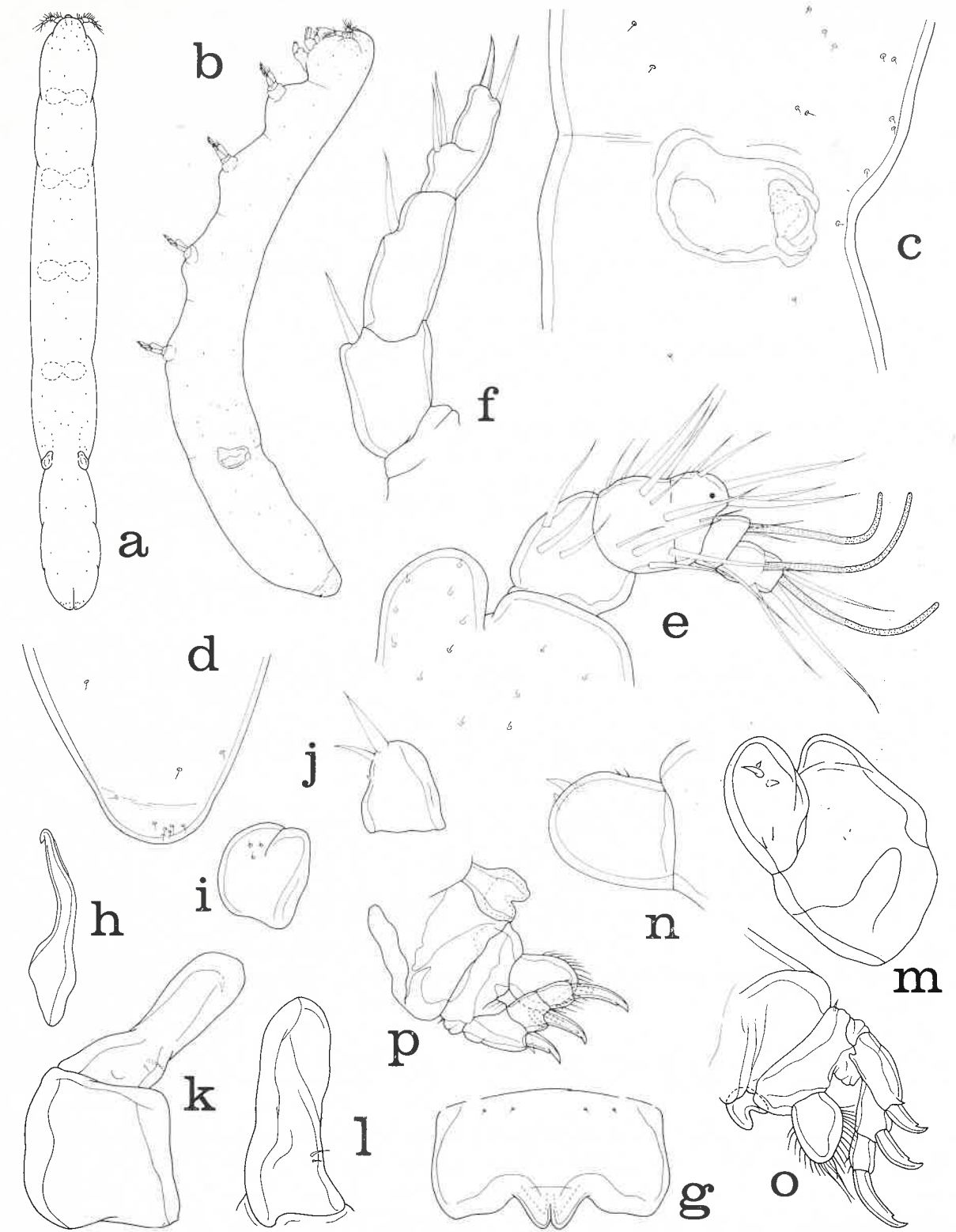
Fig. 37. Xarifia anopla n. sp., female. a, dorsal (scale B); b, lateral, (B); c, genital area, lateral (E); d, caudal ramus, lateral (E); e, rostrum and first antenna, with dot indicating position of aesthete added in male, antero-dorsal (N); f, second antenna, ventral (N); g, labrum, ventral (K); h, mandible, outer (N); i, paragnath, outer (N); j, first maxilla, ventral (N); k, second maxilla, outer (N); l, second segment of second maxilla, inner (N); m, maxilliped, antero-inner (N); n, second segment of maxilliped, anterior (N); o, leg 1 and intercoxal plate, anterior (F); p, leg 3 and intercoxal plate, posterior (F).
