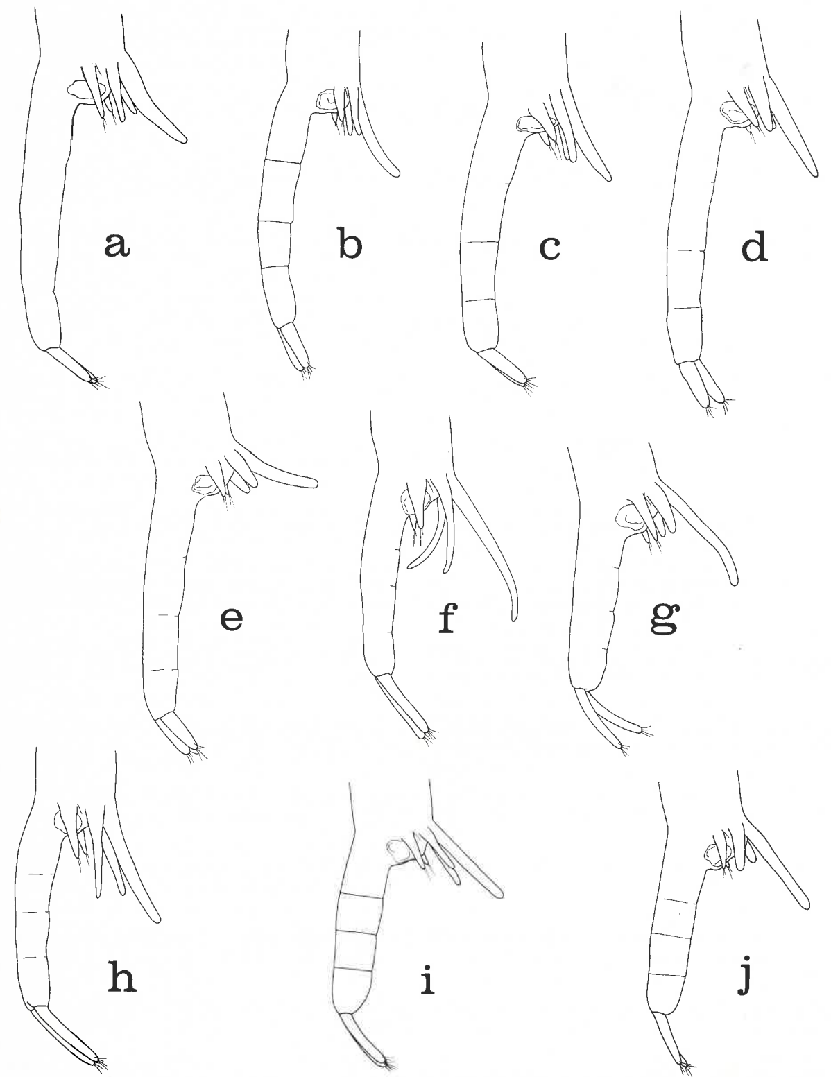
Fig. 44. Xarifia sabiuraensis Misaki, 1978. a-e, variation in urosomes of 5 females from Acropora convexa , lateral; f-j, variation in urosomes of 5 females from Acropora gravida , lateral.
