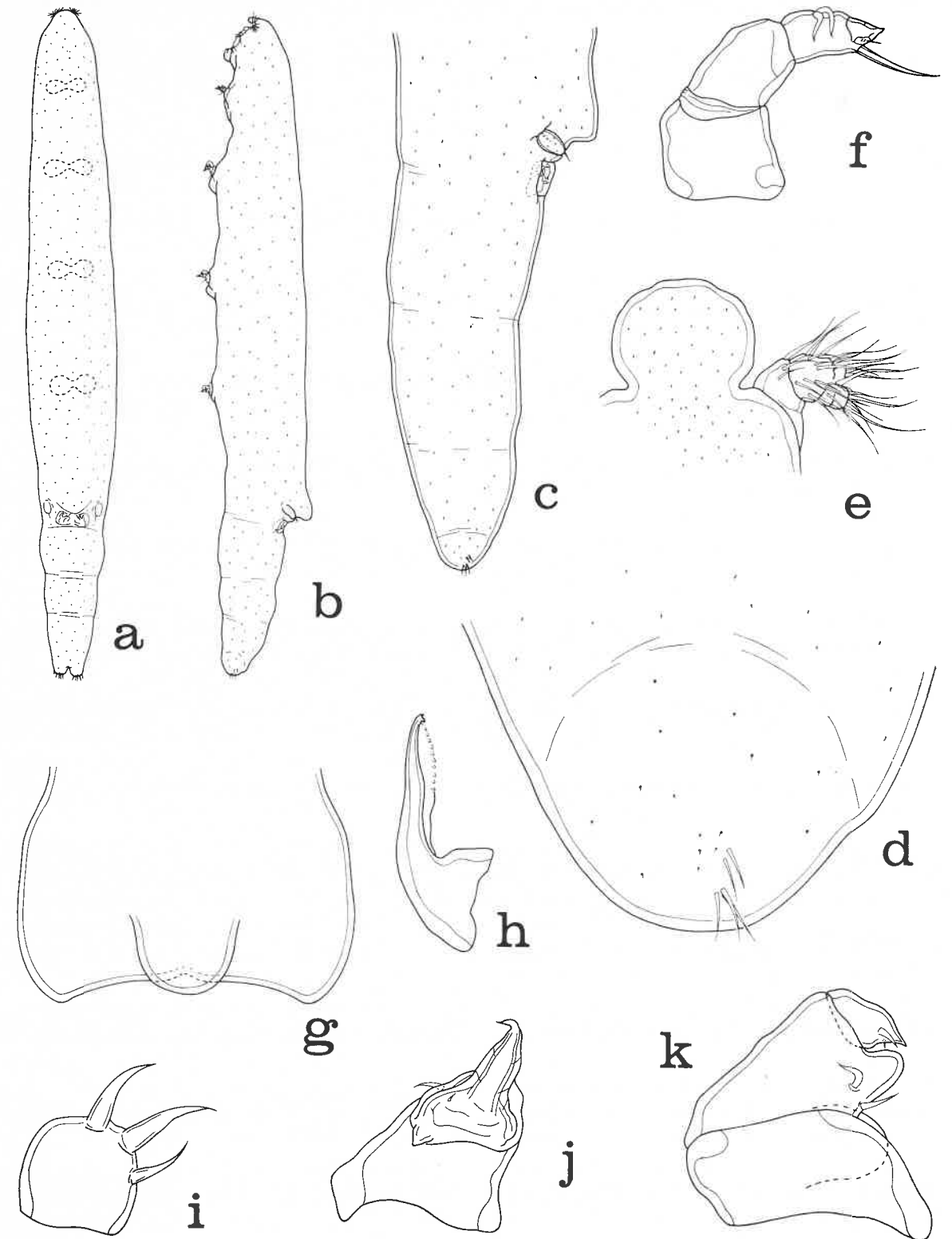
Fig. 17. Xarifia exuta n. sp., female. a, dorsal (scale A); b, lateral (A); c, urosome, lateral (E); d, caudal ramus, lateral (F); e, rostrum and first antenna, dorsal (F); f, second antenna, anteroventral (K); g, labrum, ventral (K); h, mandible, ventral (N); i, first maxilla, anteroventral (N); j, second maxilla, inner (N); k, maxilliped, inner (K).
