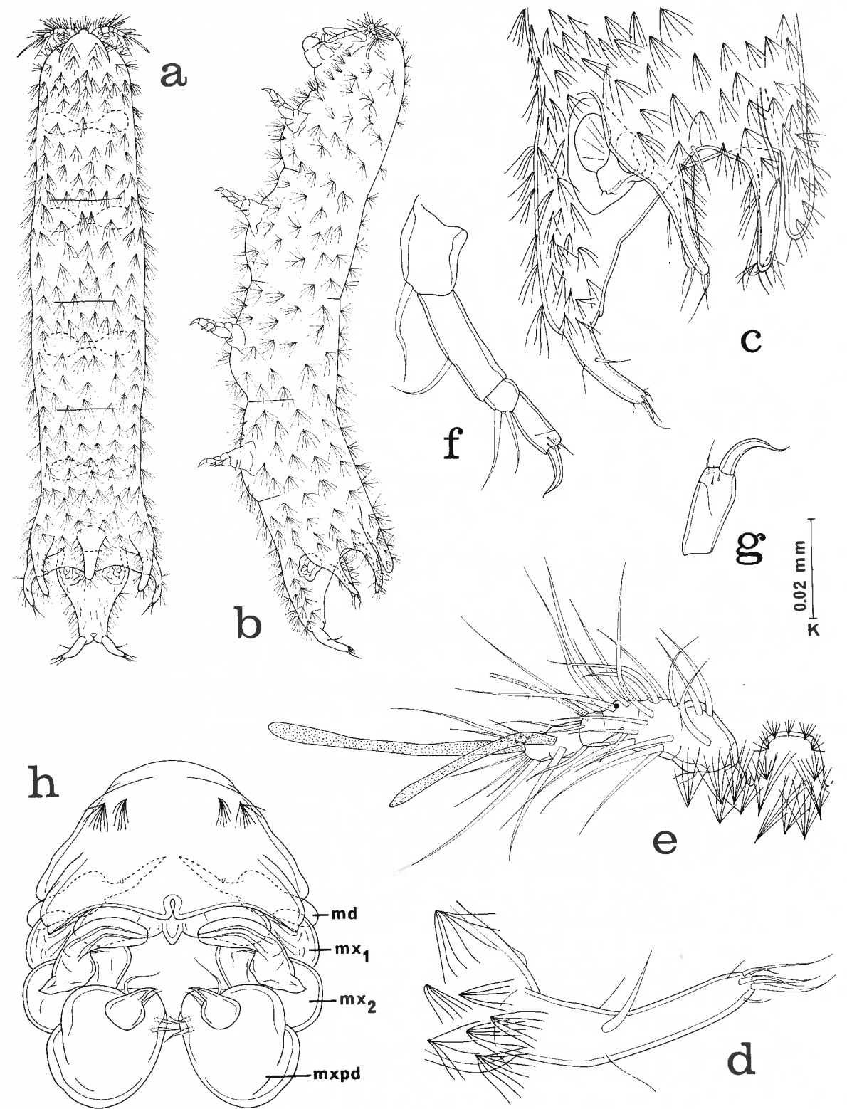
Fig. 4. Xarifia villosa n. sp., female. a, dorsal (scale B); b, lateral (B); c, urosome, lateral (I); d, caudal ramus, outer (lateral) (F); e, rostrum and first antenna, with dot indicating position of aesthete in male, anterodorsal (F); f, second antenna, dorsal (F); g, fourth segment of second antenna, dorsal (K); h, labrum, with mandibles (md), first maxillae (mx 1 ), second maxillae (mx 2 ), and maxillipeds (mxpd), ventral (F).
