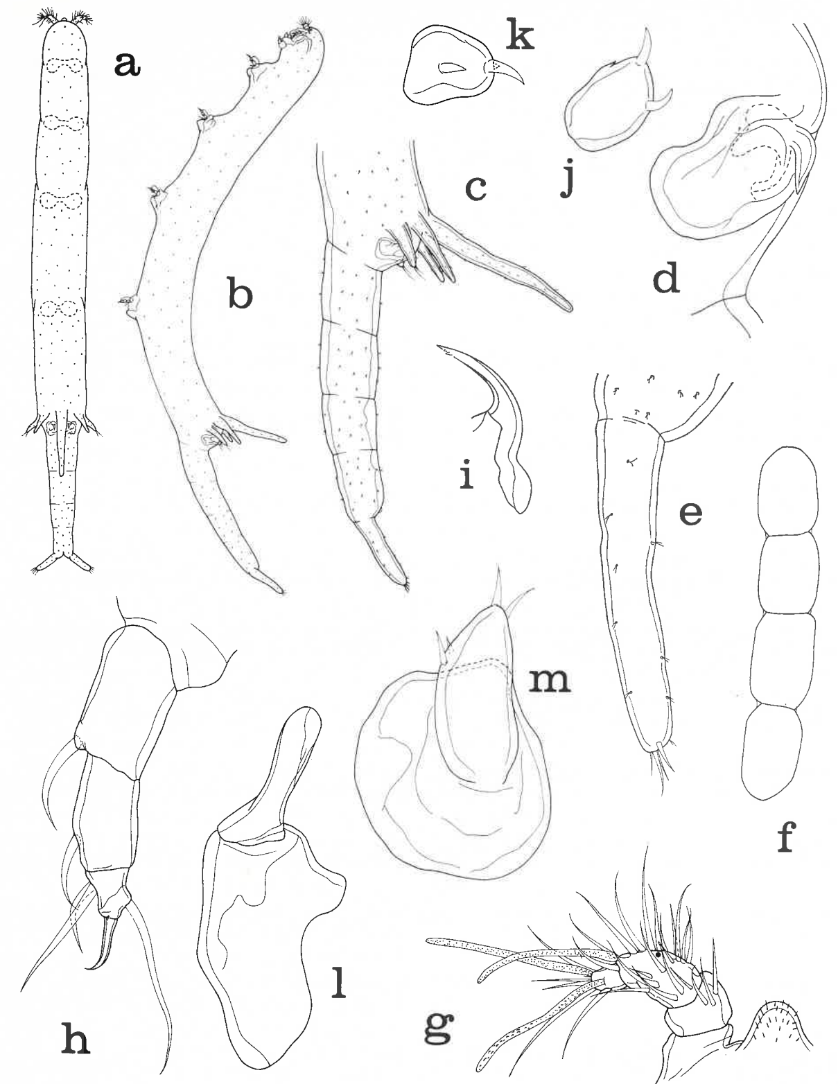
Fig. 41. Xarifia sabiuraensis Misaki, 1978, female. a, dorsal (scale M); b, lateral (M); c, urosome, lateral (J); d, genital area, lateral (F); e, caudal ramus, lateral (E); f, egg sac, lateral (B); g, rostrum and first antenna, with dot indicating position of aesthete in male, anterodorsal (F); h, second antenna, dorsal (N); i, mandible, ventral (N); j, first maxilla, outer (N); k, first maxilla, antero-inner (N); l, second maxilla, antero-inner (N); m, maxilliped, ventral (N).
