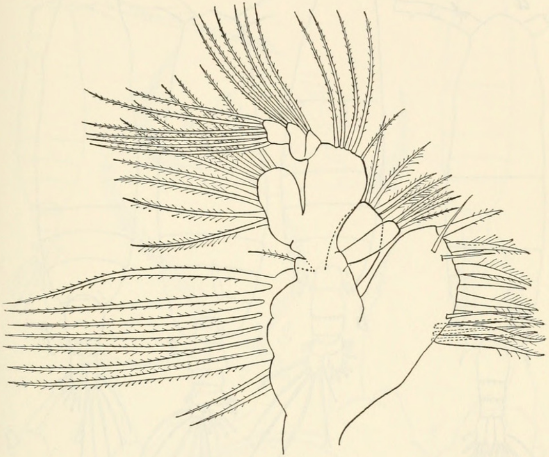
FIGURE 9.— Pseudodiaptomus cokeri , new species, female Mx1.
