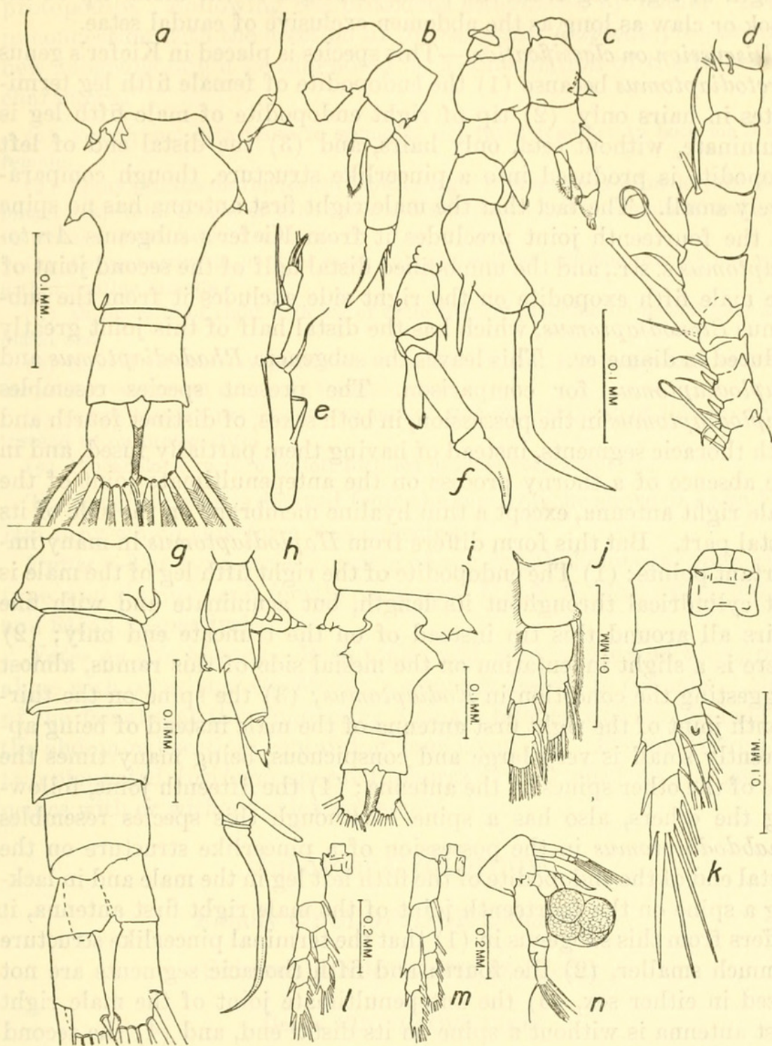
FIGURE 21.— Arctodiaptomus ( Pararctodiaptomus ) hsichowensis , new species: a , Dorsal view of abdomen of female, which has been slightly pressed to one side during mounting on slide (cf. i for more common appearance); b , fifth rudimentary leg of female; c , fifth rudimentary leg of male; d , joints 10-17 of first right antenna of male; e , last three joints of same; f , lateral view of fifth rudimentary legs of female; g , ventral view of abdomen of male; h , lateral view of fifth pair of rudimentary legs of male; i , dorsal view of last thoracic segment and abdomen of female, a commoner form than that shown in a ; j , first swimming leg of female; k-m , second to fourth swimming legs of male; n , lateral view of posterior end of female showing ovipositor with four eggs.
