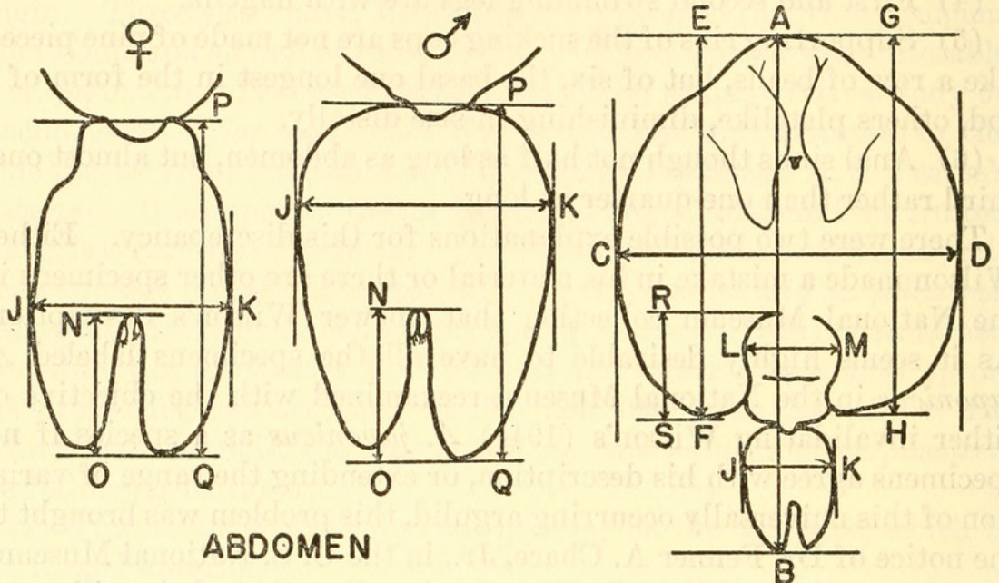
FIGURE 26.—Method used for measuring Argulus japonicus : AB, total length; CD, maximum width; EF, length of left carapace; GH, length of right carapace; JK, width of abdomen; LM, maximum width of posterior sinus of carapace; NO, length of anal sinus; PQ, length of abdomen; RS, length of posterior sinus of carapace.
