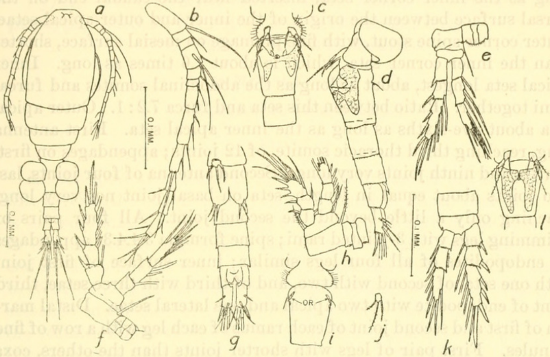
FIGURE 23.— Tropocyclops breviramus , new species: a, Female, dorsal view; b, first antenna of female; c, genital segment of female, ventral view; d, same, lateral view; e, fourth leg of female; f, third leg of female; g, abdomen of male, dorsal view; h, first leg of female; i, genital segment of female, dorsal view; j, fifth rudimentary leg of female; k, second leg of female; l, genital segment of female, ventral view.
