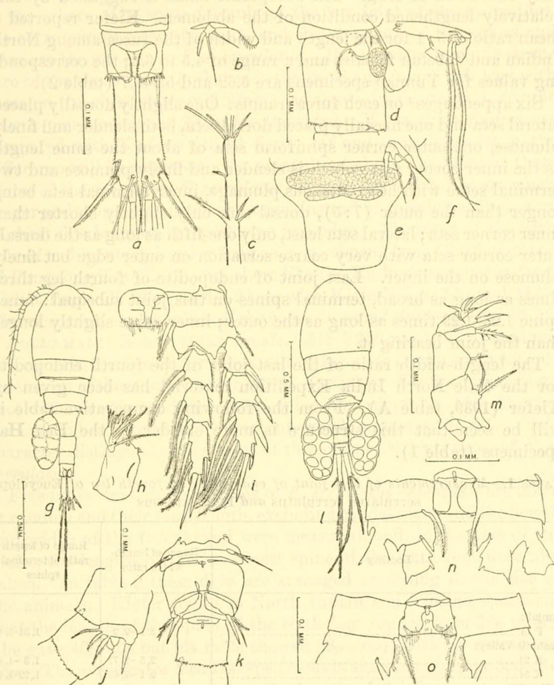
FIGURE 22.— Eucyllops serrulatus extensus , new subspecies: a , Furcal rami and last abdominal (anal) segment of female, dorsal view; b , fifth leg of female; c , last joint of first antenna of female; d , genital segment of female, lateral view showing spermatophores and fifth and sixth legs; e , ventral view of genital segment of female showing receptaculum seminis; f , mandible of female showing elongated setae; g , dorsal view of female with one ovigiger and one antenna removed; h , maxilla of female; i , fourth leg of female; j , genital segment of male showing sixth leg, lateral view; k , same, ventral view; l , dorsal view of E. s. serrulatus from Leh, Ladak (L 13); m , anterior maxilliped of female; n , base of fourth pair of legs of E. s. serrulatus (Fischer) from Kashmir, Yale North India Expedition, station K 35; o , same of E. s. extensus from Lake Erh Hai.
