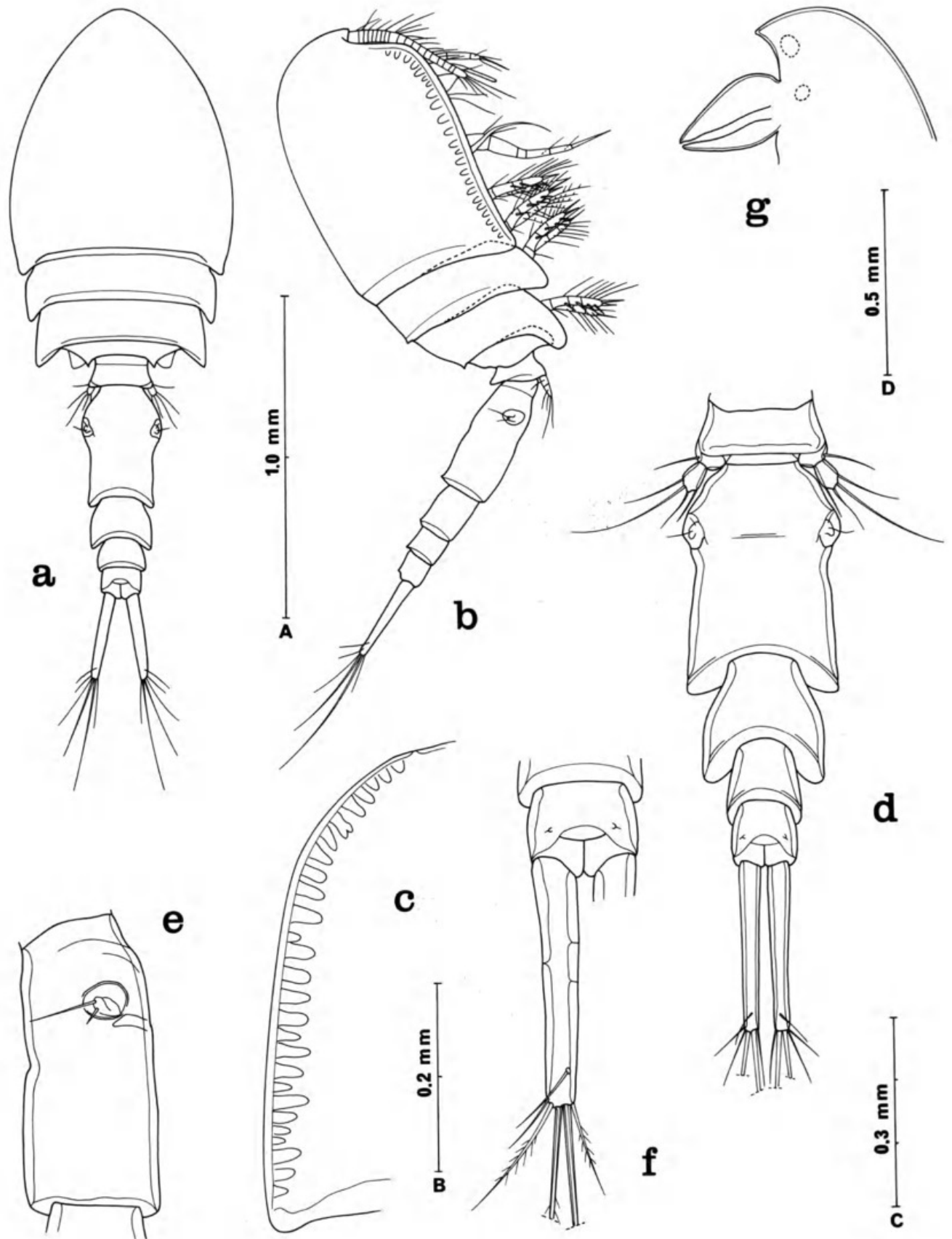
FIG. 1. — Cheramomyzon abyssale n. gen., n. sp., female : a, dorsal (scale A); b, lateral (A); c, edge of cephalosoma, ventral (B); d, urosome, dorsal (C); e, genital segment, lateral (B); f, anal segment and caudal ramus, dorsal (B); g, outline of rostrum and oral cone, lateral (D).
