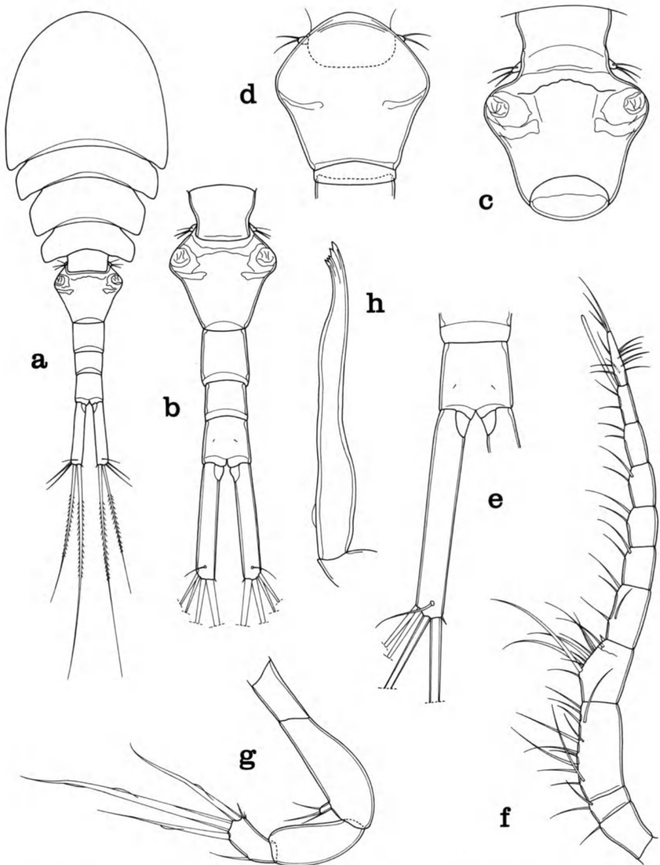
FIG. 6. — Benthoxynus tumidiseta n. sp., female : a, dorsal (scale D); b, urosome, dorsal (C); c, segment bearing leg 5 and genital segment, dorsal (B); d, genital segment, ventral (B); e, anal segment and caudal ramus, dorsal (B); f, first antenna, ventral (B); g, second antenna, postero-outer (E); h, mandible, posterior (G).
