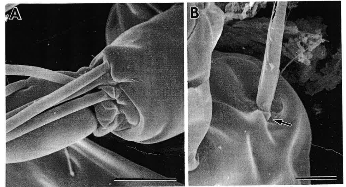
Fig. 25. Metacalanus sp. 1, female (A); Metacalanus sp. 2, female (B). SEM micrographs of mouthparts. A, Detail of segments IV to VIII of antennary exopod, scale bar = 10 \mu\text{m} ; B, Mandibular endopod, indicated by arrow, scale bar = 5 \mu\text{m} .
