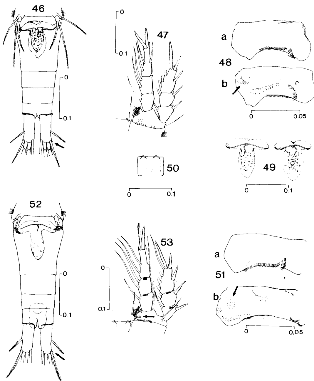
Figs 46–53. 46–50 Mesocyclops c.f. thermocyclopioides 46 abdominal segments with seminal receptacle and furca, 47 fourth leg, 48 basipodite of antenna (a.: frontal view, b.: caudal view), 49 variations in seminal receptacles, 50 connecting lamella of fourth leg, 51–53 Mesocyclops thermocyclopoides (s. str.), 51 basipodite of antenna (a.: frontal view, b.: caudal view), 52 abdominal segments with seminal receptacle and furca, 53 fourth leg. (scales are in mm).
