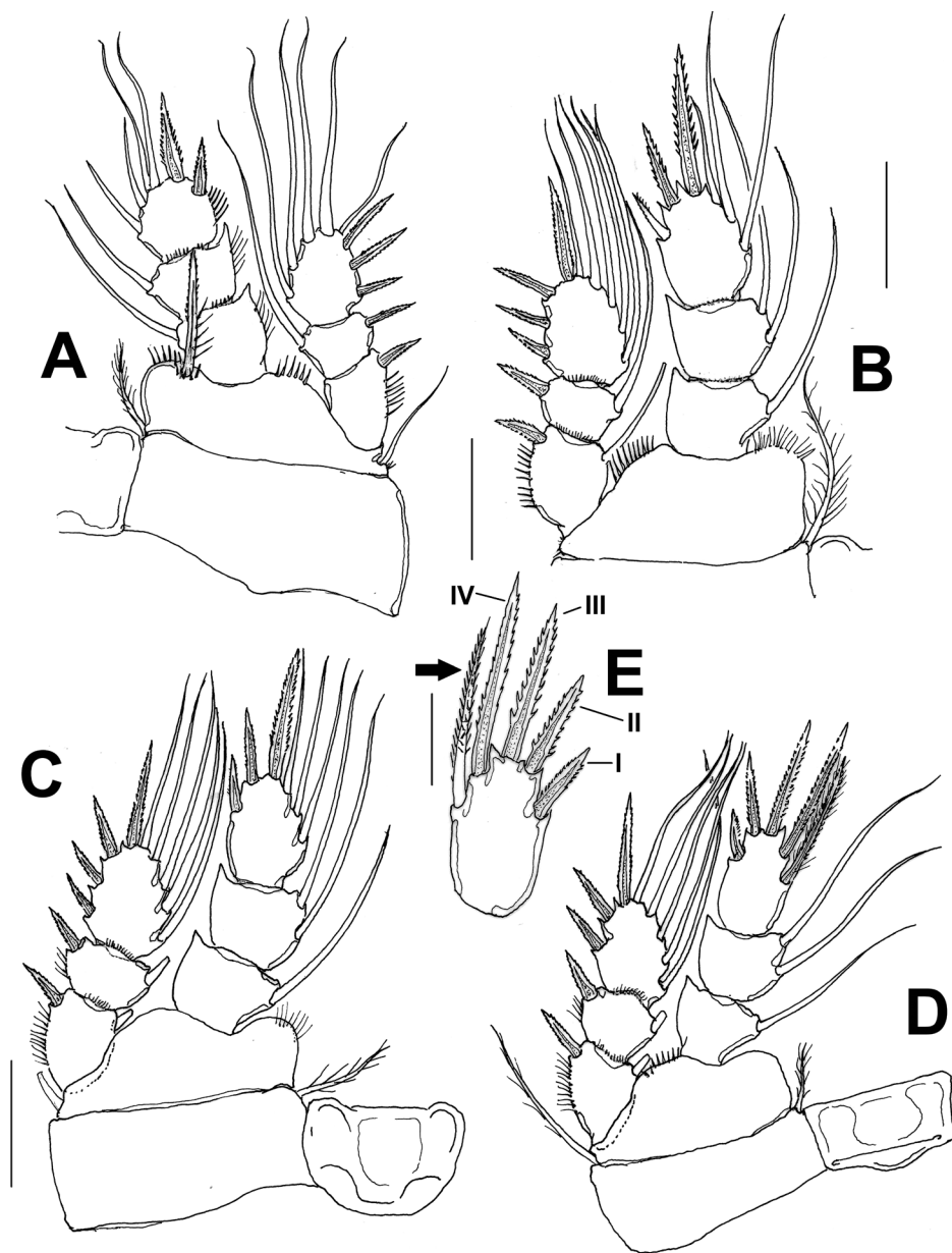
Figure 2. Halicyclops gaviriai sp. n., adult holotype female from northern Colombia. A leg 1 B leg 2 C leg 3 D leg 4 E . leg 4 terminal endopodal segment showing details of armature. Scale bars: A–D = 50 µm, E =25 µm.
