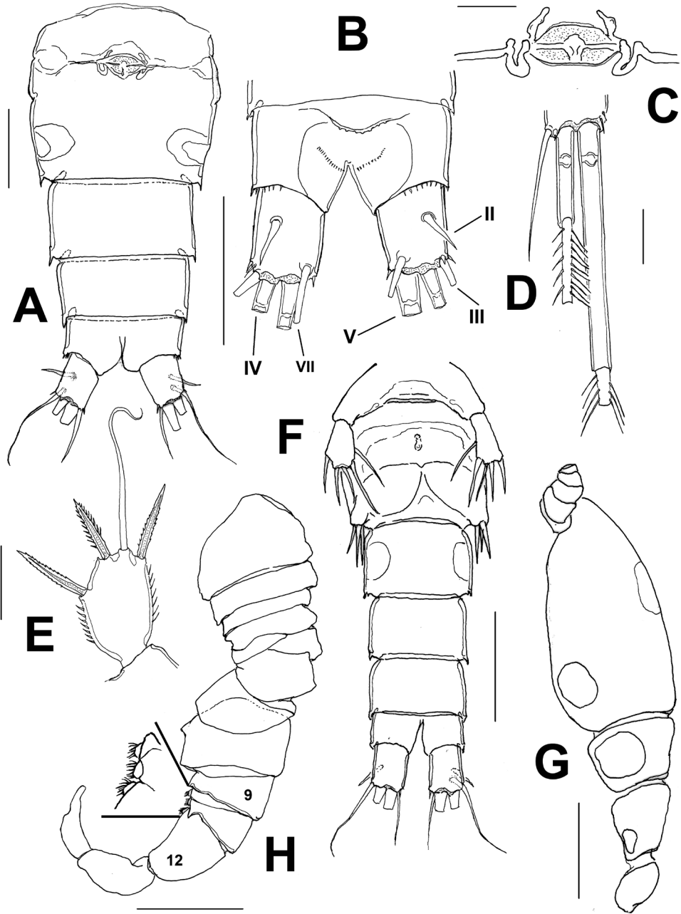
Figure 3. Halicyclops gaviriai sp. n., adult holotype female from northern Colombia. A urosome showing genital somite, ventral view B anal somite showing anal pseudopericulum, dorsal view C internal structures of genitalia, ventral view D proximal section of middle apical setae of caudal ramus E leg 5; adult male from same locality F urosome, ventral view G lateral view of cephalothorax showing position of integumental windows H geniculate antennule, showing brush-like modified setae on segments 10–12. Scale bars: A, B, F, H = 50 \mu m, C–E = 25 \mu m, G = 100 \mu m.
