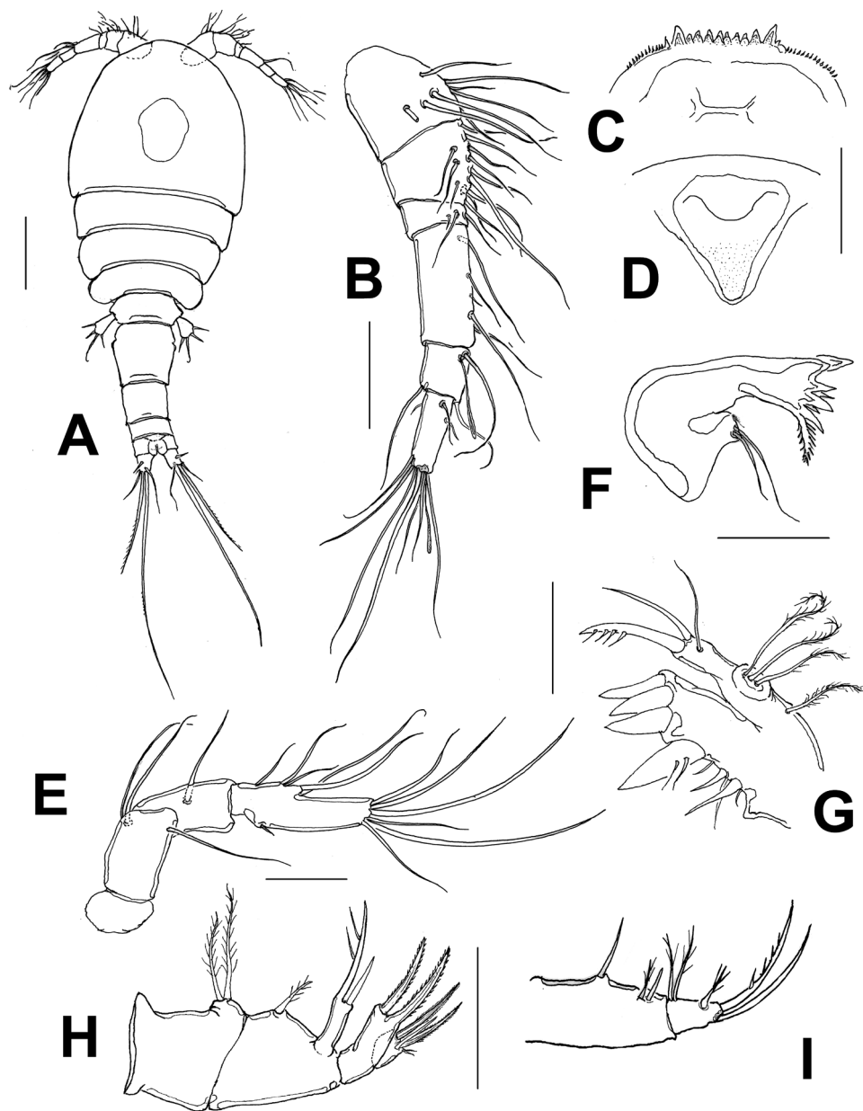
Figure 1. Halicyclops gaviriai sp. n., adult paratype female from northern Colombia. A habitus, dorsal view B antennule C labrum, ventral D rostrum E antenna F mandible G maxillule H maxilla I maxilliped. Scale bars: A =100 µm, B–F = 50 µm.
