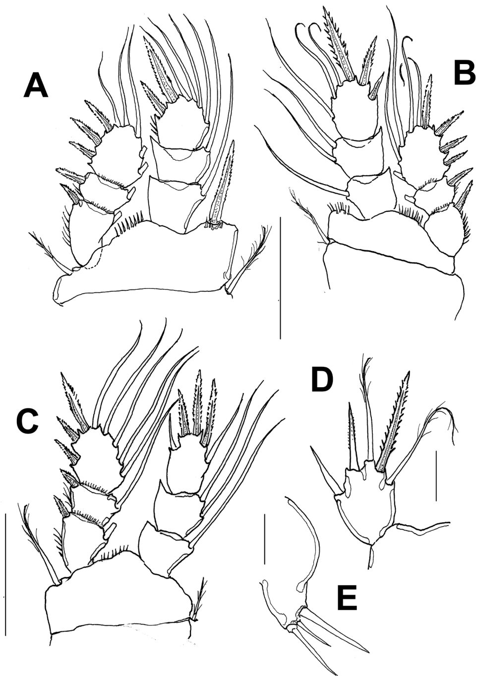
Figure 4. Halicyclops gaviriai sp. n., adult male allotype from northern Colombia. A leg 1 B leg 2 C leg 4 D leg 5 E leg 6. Scale bars: A–C = 50 \mu m, D =25 \mu m, E = 10 \mu m.
