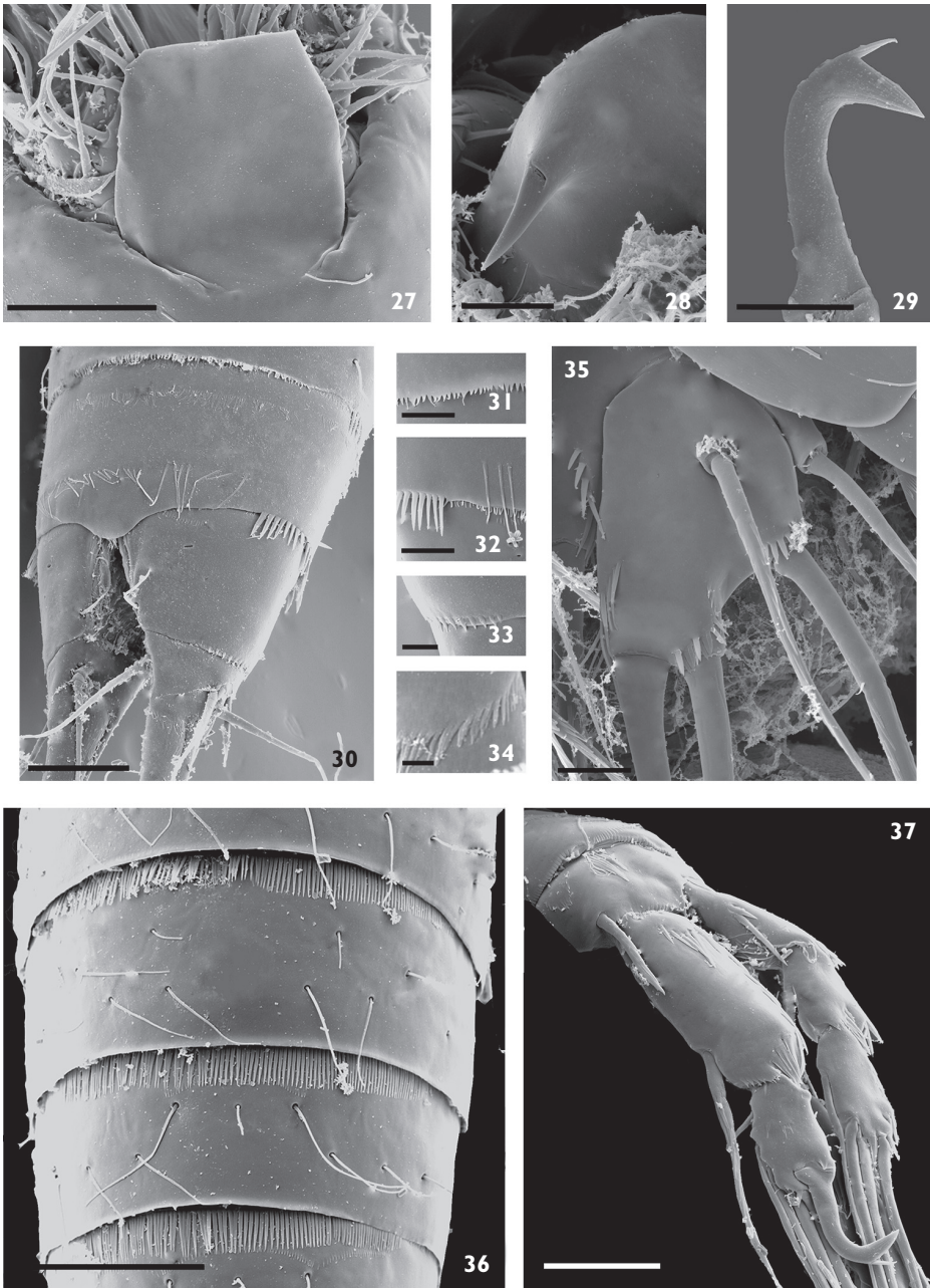
Figures 27-37. Chaulionyx paivacarvalhoi gen. et sp. n. Scanning electron micrographs (♀: 27-35 ; ♂: 36-37 ): 27 rostrum, dorsal 28 labrum, anterior 29 bifid outer spine on P1 enp-2 30 second abdominal somite (posterior margin), third abdominal somite, anal somite and caudal rami, dorsolateral 31 detail of serrate posterior margin of second abdominal somite 32 detail of posterior margin of third abdominal somite 33 posterior margin of anal somite 34 posterior margin of caudal ramus showing dorsal semi-circular serrate extension 35 P5, anterior 36 prosomal ornamentation, dorsal 37 P1 endopod, anterior. Scale bars: 1 µm ( 34 ), 2.5 µm ( 33 ), 5 µm ( 28-29 , 31-32 , 35 ), 10 µm 27 ( 30 , 37 ), 20 µm ( 36 ).
