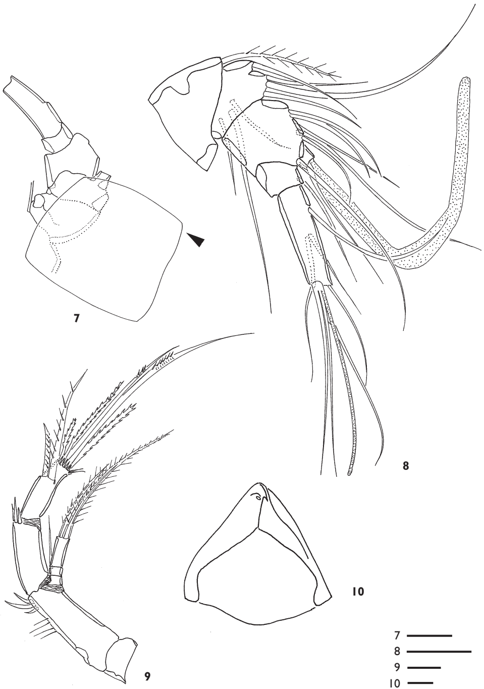
Figures 7-10. Chaulionyx paivacarvalhoi gen. et sp. n. ♀: 7 rostrum (arrowed) and left antennule (armature omitted), dorsal 8 right antennule, dorsal 9 antenna 10 labrum. Scale bars = 10 µm.
