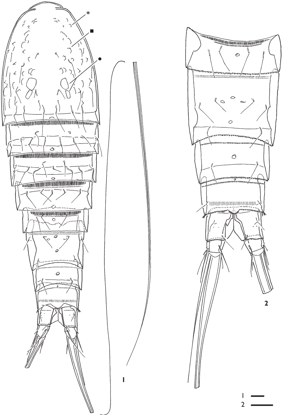
Figures 1-2. Chaulionyx paivacarvalhoi sp. n. ♀: 1 habitus, dorsal [* = integumental pit; ■ = pore ; ● = chitinous patch 2 urosome, dorsal. Scale bars = 10 µm.
