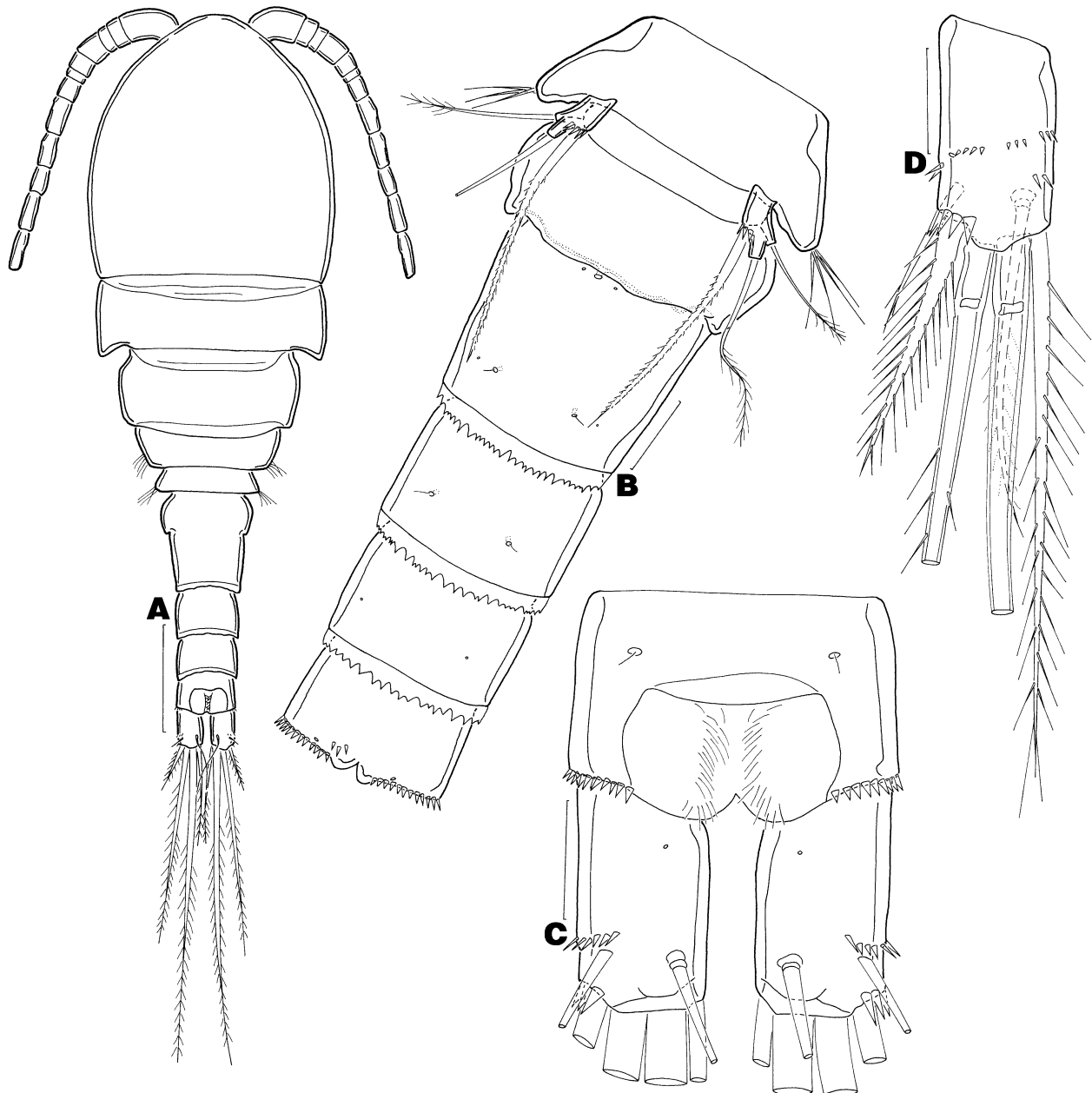
FIGURE 2. Eucyclops edytæ sp. nov., adult female. (A) habitus, dorsal; (B) urosome, ventral; (C) anal somite and caudal rami, dorsal; (D) caudal ramus, ventral. Scale bars: A, 100 µm; B, 25 µm; C–D, 20 µm.
