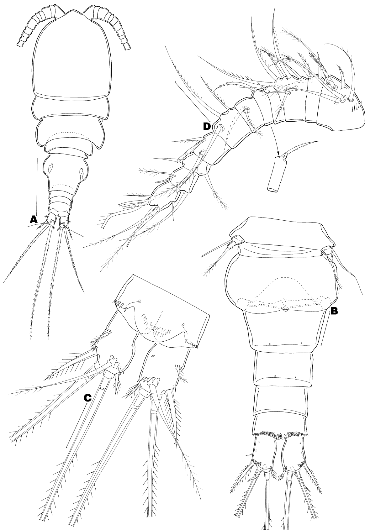
FIGURE 22. Mixocyclops mortoni sp. nov. , adult female. (A) habitus, dorsal; (B) urosome, ventral; (C) anal somite and caudal rami, dorsal; (D) antennule, ventral (with dorsal view of segment 5 shown separately). Scale bars: A, 100 \mu m; B, D, 25 \mu m; C, 20 \mu m.
