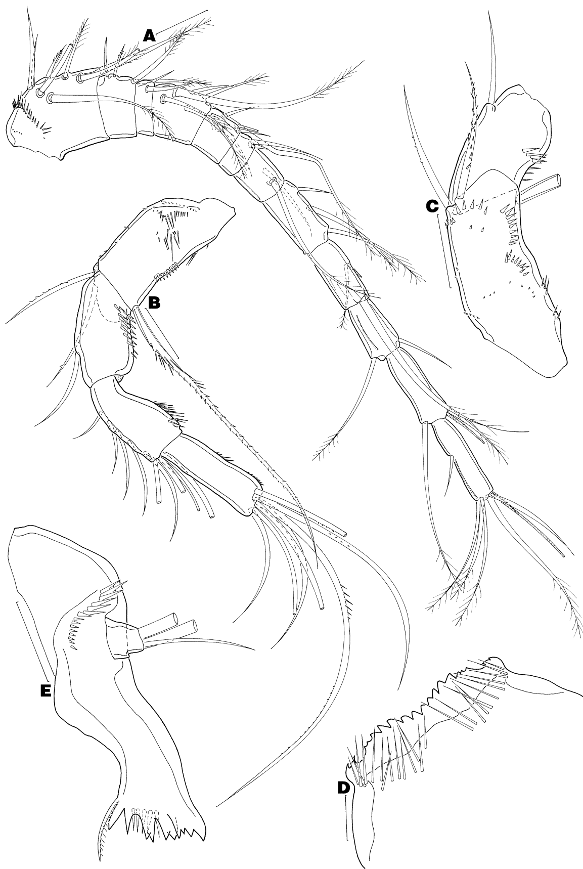
FIGURE 3. Eucyclops edytæ sp. nov., adult female. (A) antennule, ventral; (B) antenna, frontal; (C) antennal coxobasis and proximal endopodal segment, caudal; (D) labrum, anterior; (E) mandible, posterior. Scale bars: A, 25 µm; B–C, E, 20 µm; D, 10 µm.
