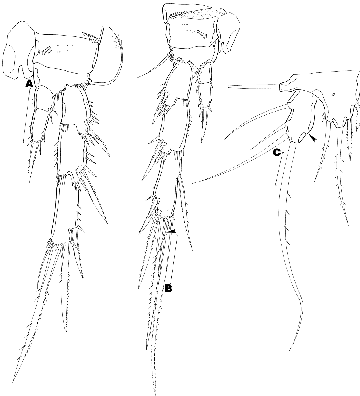
FIGURE 29. Paranitocrella bastiani gen. et sp. nov. , adult female. (A) leg 3, anterior; (B) leg 4 (inner apical seta indicated by arrowhead), anterior; (C) leg 5 (position of cuticular pore opening indicated by arrowhead), ventral. Scale bars: A–B, 20 \mu m; C, 10 \mu m.
