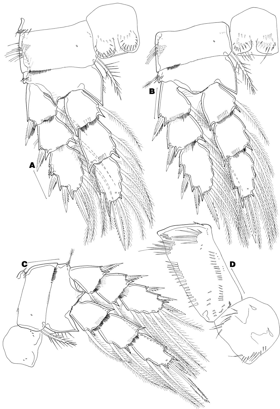
FIGURE 5. Eucyclops edytae sp. nov. , adult female. (A) leg 2, anterior; (B) leg 3, anterior; (C) leg 4, anterior; (D) leg 4 intercoxal sclerite and coxa, posterior. Scale bars: A–C, 25 \mu m; D, 15 \mu m.
