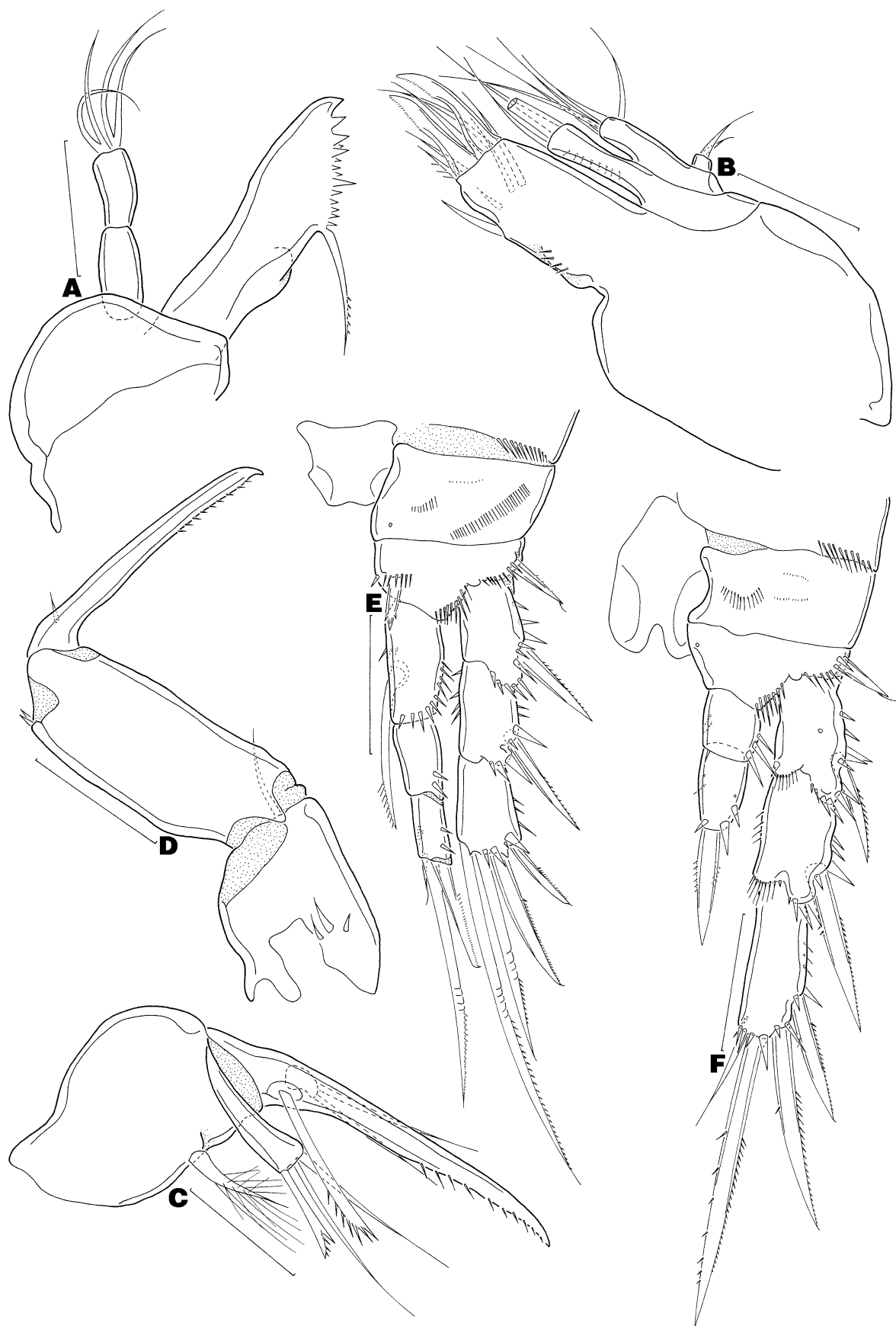
FIGURE 28. Paranitocrella bastiani gen. et sp. nov. , adult female. (A) mandible, anterior; (B) maxillule, posterior; (C) maxilla, anterior; (D) maxilliped, posterior; (E) leg 1, anterior; (F) leg 2, anterior. Scale bars: A–D, 10 \mu m; E–F, 20 \mu m.
