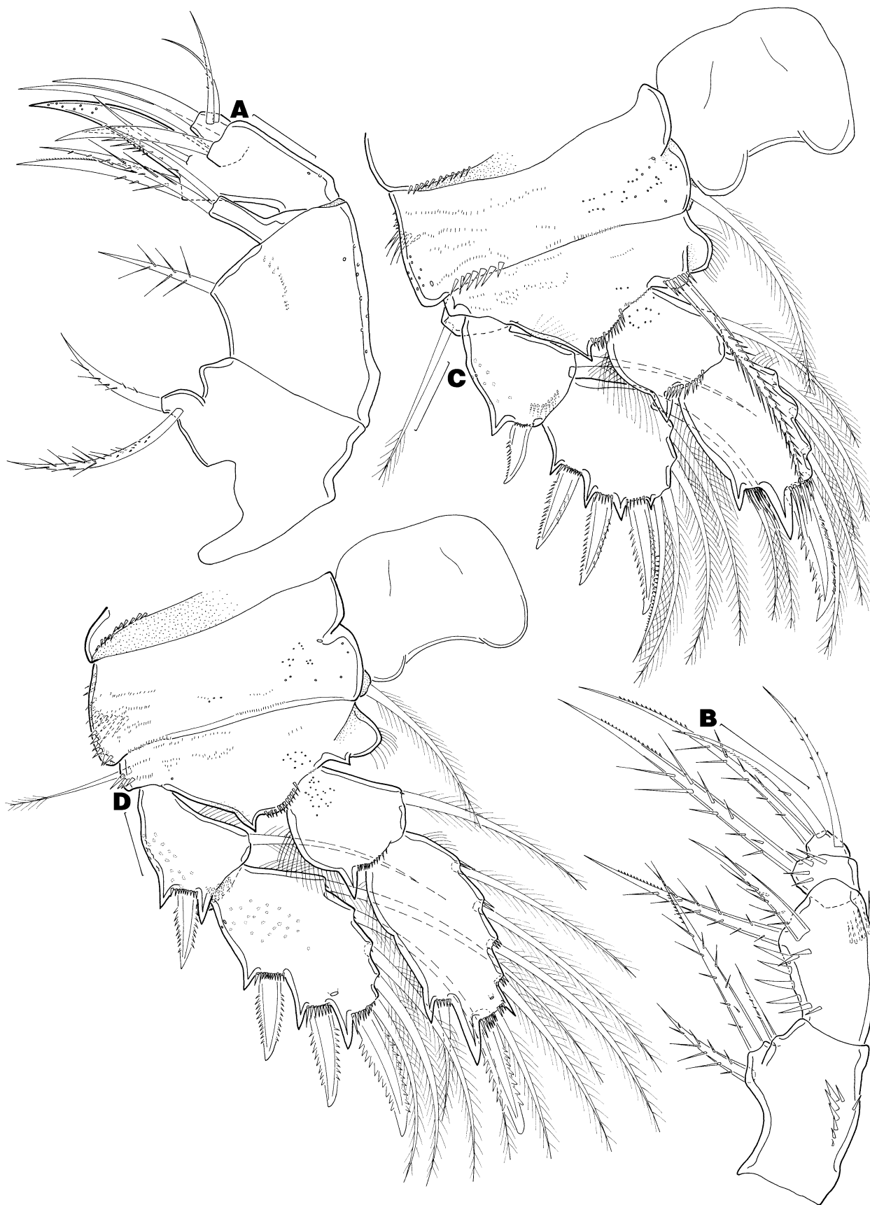
FIGURE 19. Metacyclops arnaudi (G. O. Sars, 1908), adult female. (A) maxilla, posterior; (B) maxilliped, anterior; (C) leg 1, anterior; (D) leg 2, anterior. Scale bars: A–D, 20 \mu m.
