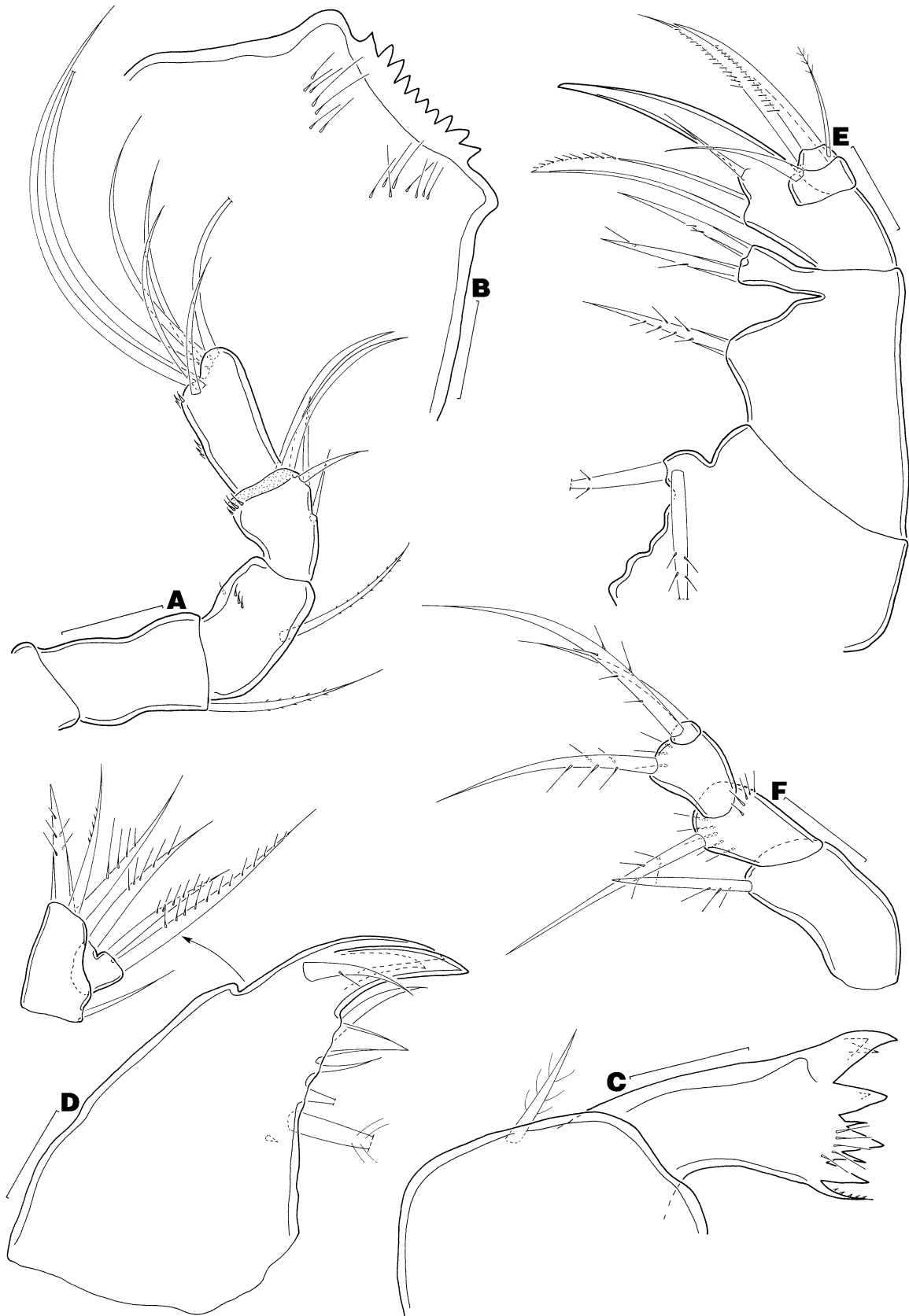
FIGURE 23. Mixocyclops mortoni sp. nov. , adult female. (A) antenna, frontal; (B) labrum, anterior; (C) mandible, anterior; (D) maxillule with palp disarticulated from coxa, posterior; (E) maxilla, posterior; (F) maxilliped, posterior. Scale bars: A, 15 \mu m; B–F, 10 \mu m.
