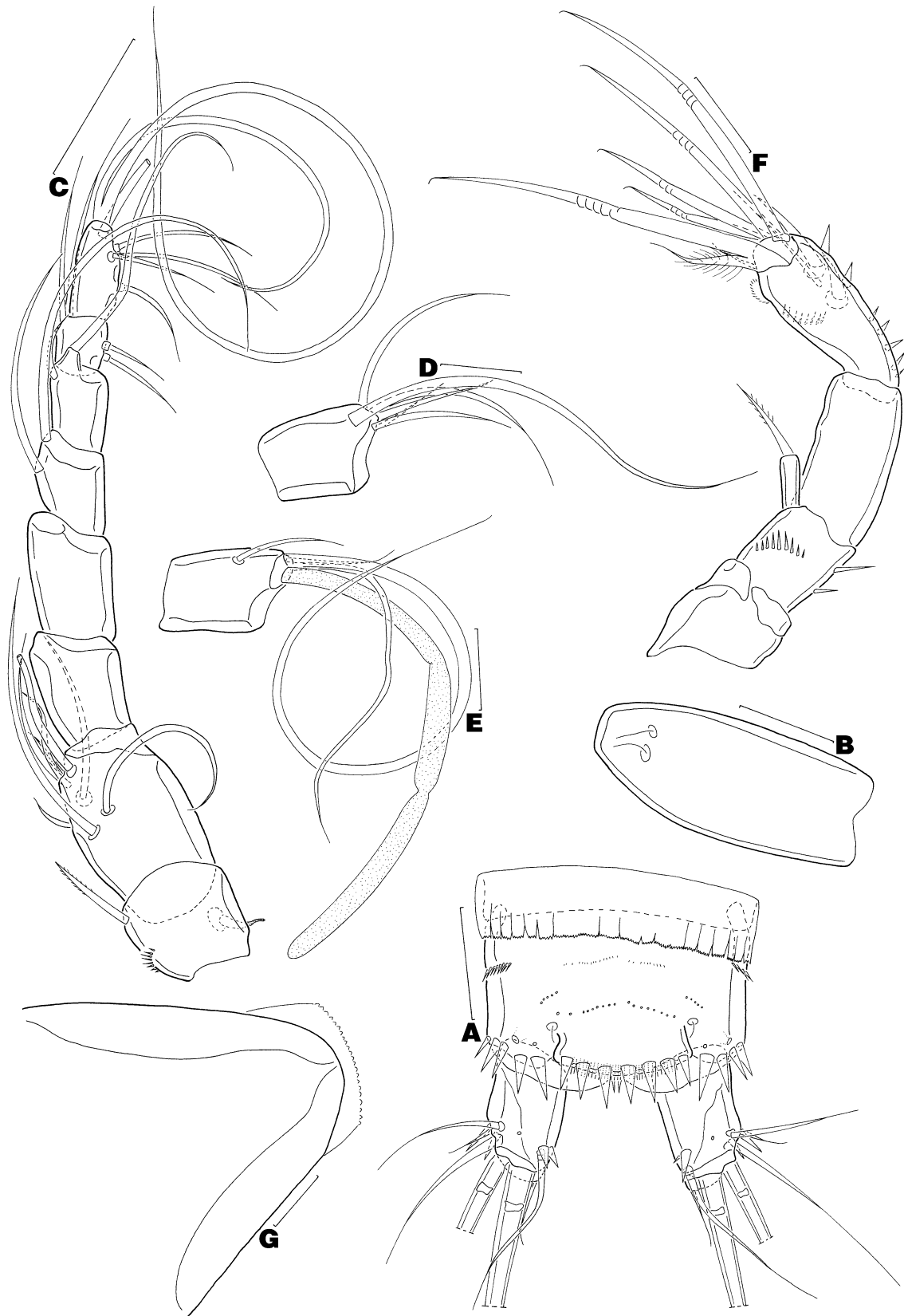
FIGURE 27. Paranitocrella bastiani gen. et sp. nov. , adult female. (A) anal somite and caudal rami, dorsal; (B) rostrum, dorsal; (C) antennule (armature omitted on segments 3 and 4), ventral; (D) antennular segment 3, ventral; (E) antennular segment 4, ventral; (F) antenna, anterolateral; (G) labrum, anterior. Scale bars: A, C, 20 \mu m; B, G, 5 \mu m; D–F, 10 \mu m.
