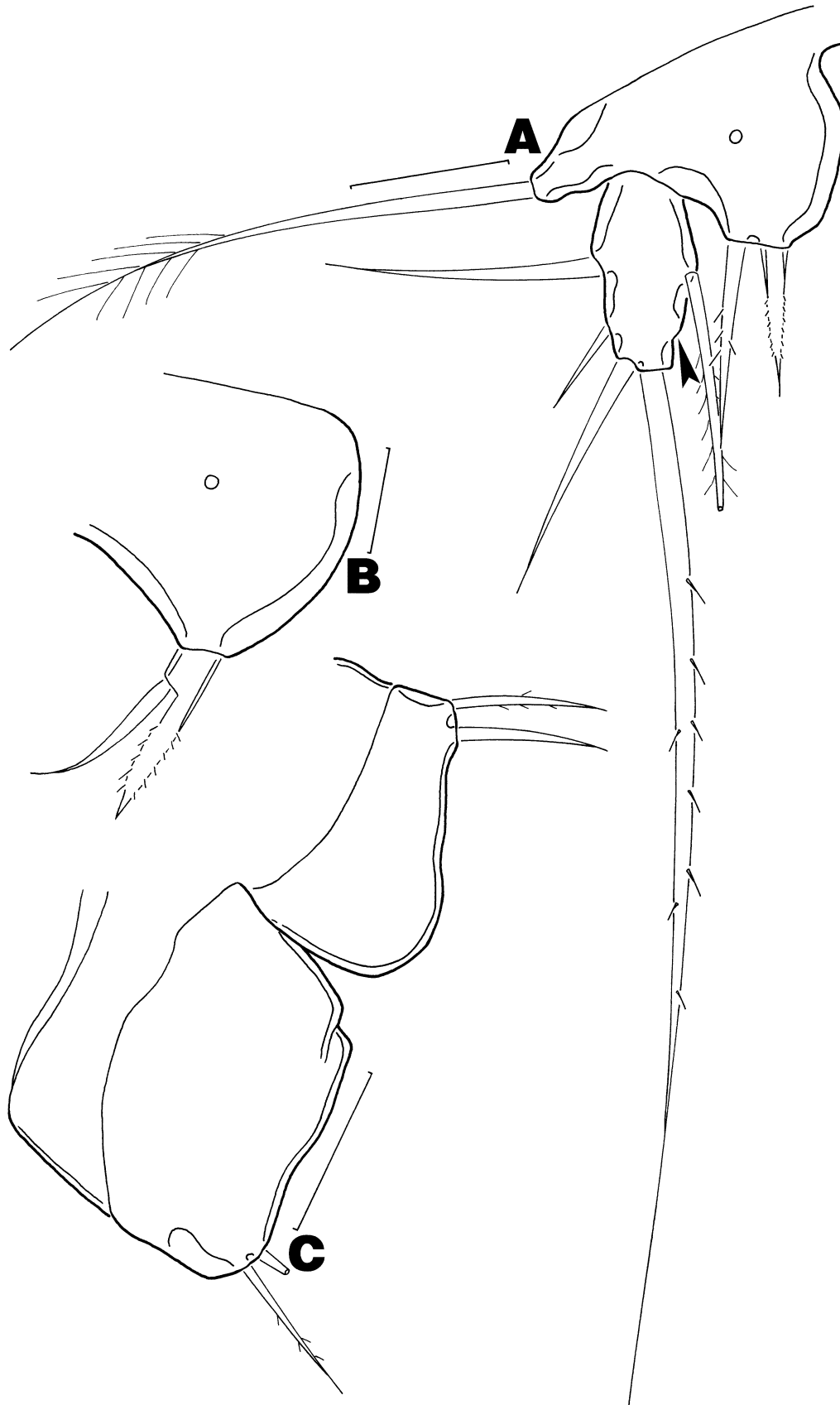
FIGURE 31. Paranitocrella bastiani gen. et sp. nov. , adult male. (A) leg 5 (position of cuticular pore opening indicated by arrowhead), ventral; (B) abnormal leg 5 basoendopod, ventral; (C) leg 6, ventral. Scale bars: A, C, 10 \mu m; B, 5 \mu m.
