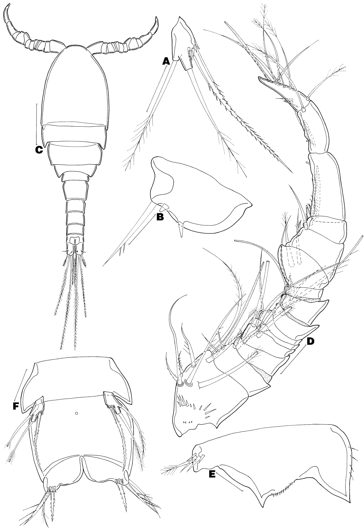
FIGURE 6. Eucyclops edytæ sp. nov. , adult female (A–B) and adult male (C–F). (A) leg 5, ventral; (B) leg 6, lateral; (C) habitus, dorsal; (D) antennule, ventral; (E) leg 3 basis, anterior; (F) urosomites 1 and 2 showing legs 5 and 6, ventral. Scale bars: A, D, F, 20 \mu m; B, E, 10 \mu m; C, 100 \mu m.
