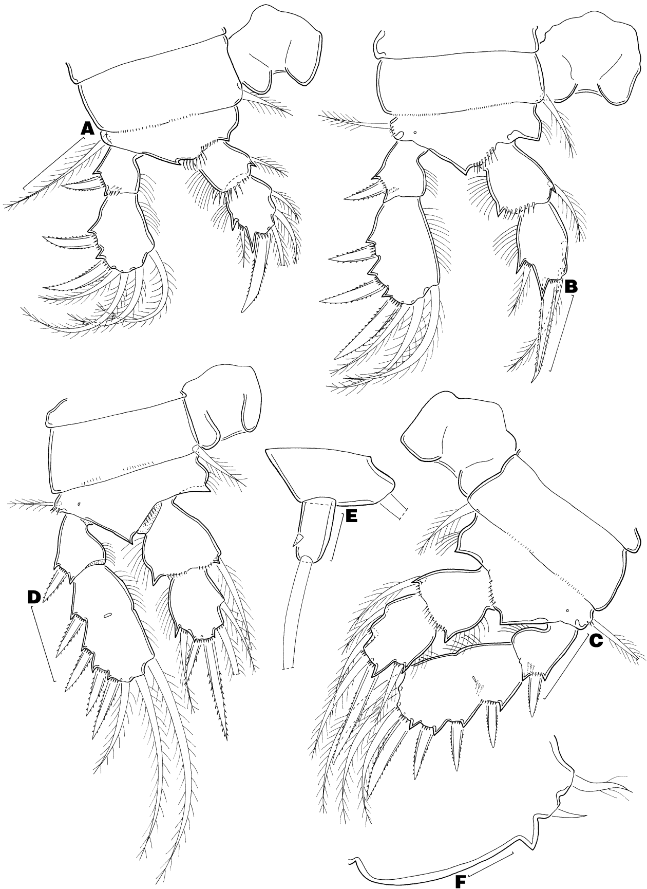
FIGURE 24. Mixocyclops mortoni sp. nov. , adult female. (A) leg 1, anterior; (B) leg 2, anterior; (C) leg 3, anterior; (D) leg 4, anterior; (E) leg 5, ventrolateral; (F) leg 6, dorsolateral. Scale bars: A–D, 20 µm; E–F, 5 µm.
