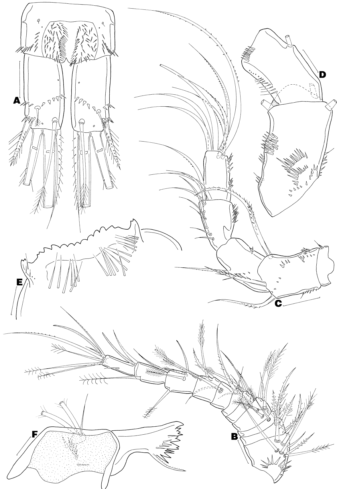
FIGURE 8. Paracyclops intermedius sp. nov. , adult female. (A) anal somite and caudal rami, dorsal; (B) antennule, ventral; (C) antenna, caudal; (D) antennal coxobasis and proximal endopodal segment, frontal; (E) labrum, anterior; (F) mandible, anterior. Scale bars: A, 25 \mu m; B–C, 20 \mu m; D–F, 10 \mu m.
