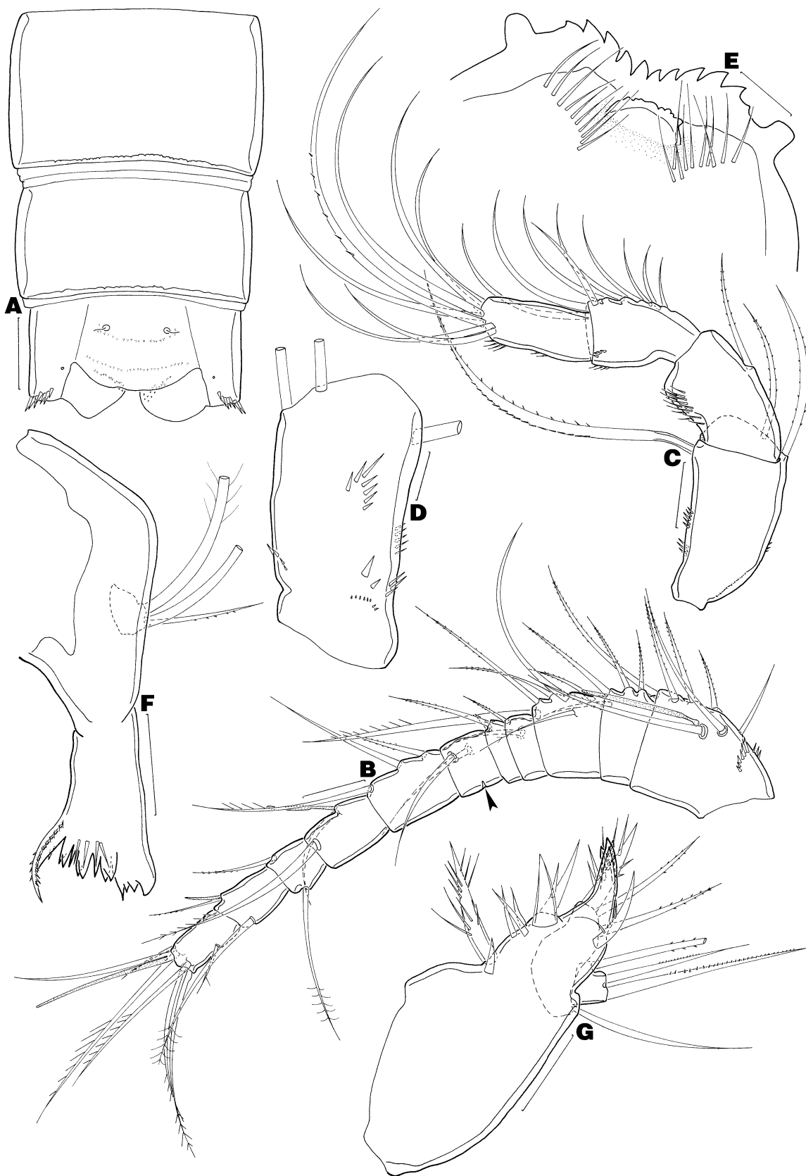
FIGURE 18. Metacyclops arnaudi (G. O. Sars, 1908), adult female. (A) postgenital somites, dorsal; (B) antennule (partial articulation indicated by arrowhead), ventral; (C) antenna, frontal; (D) antennal coxobasis, caudal; (E) labrum, anterior; (F) mandible, anterior; (G) maxillule, posterior. Scale bars: A, C, F, G, 20 \mu m; B, 25 \mu m; D–E, 10 \mu m.
