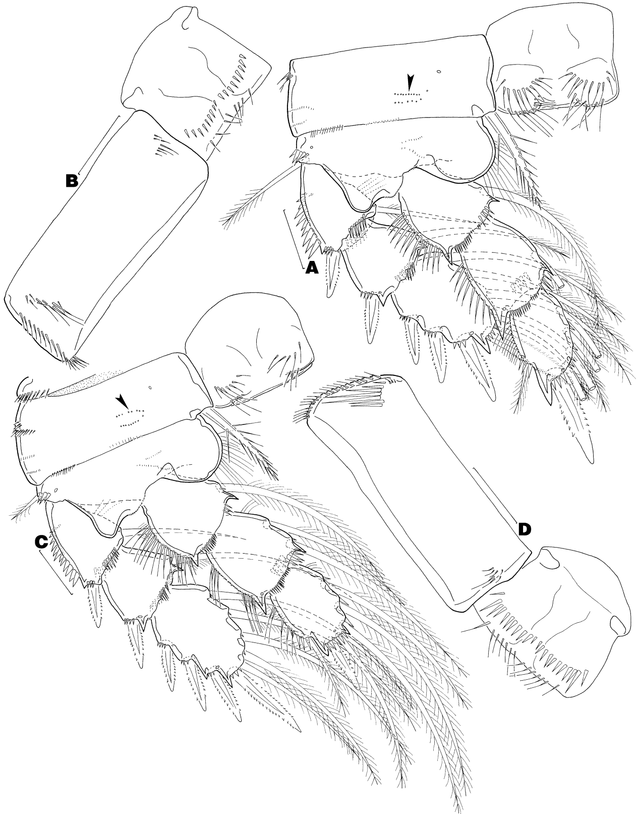
FIGURE 10. Paracyclops intermedius sp. nov. , adult female. (A) leg 2 (sockets of spinules indicated by arrowhead), anterior; (B) leg 2 intercoxal sclerite and coxa, posterior; (C) leg 3 (sockets of spinules indicated by arrowhead), anterior; (D) leg 3 intercoxal sclerite and coxa posterior. Scale bars: A–D, 20 \mu m.
