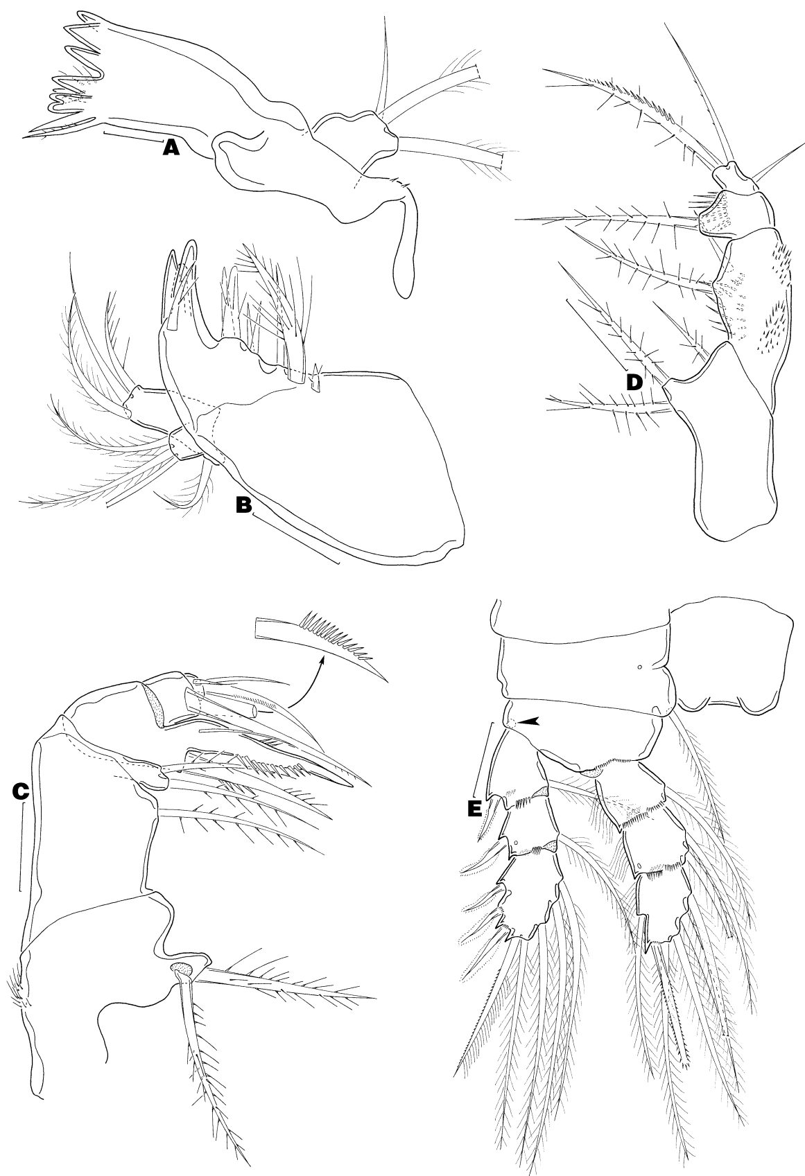
FIGURE 14. Tropocyclops confinis (Kiefer, 1930), adult female. (A) mandible, anterior; (B) maxillule, posterior; (C) maxilla with anterodistal element on proximal endopodal segment shown separately, posterior; (D) maxilliped, posterior; (E) leg 1 (socket of missing seta indicated by arrowhead), anterior. Scale bars: A, 10 \mu\text{m} ; B–D, 20 \mu\text{m} ; E, 25 \mu\text{m} .
