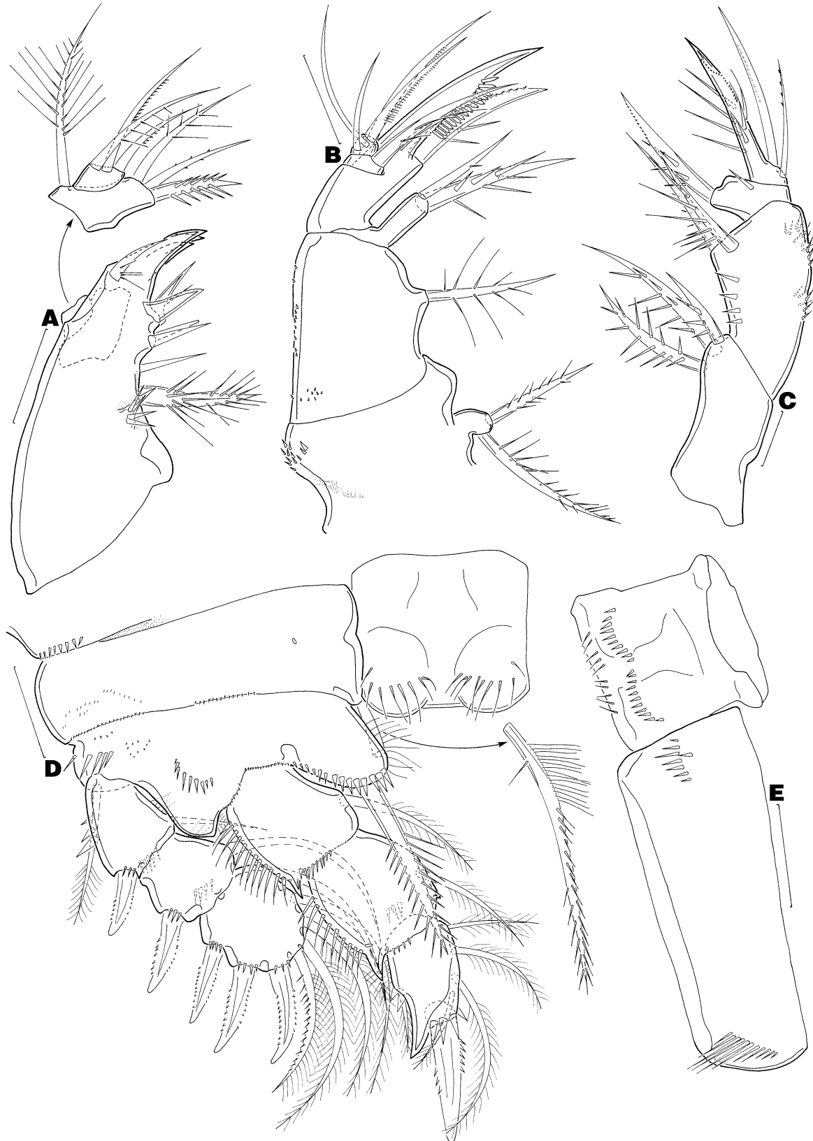
FIGURE 9. Paracyclops intermedius sp. nov. , adult female. (A) maxillule with palp disarticulated from coxa, posterior; (B) maxilla, posterior; (C) maxilliped, anterior; (D) leg 1 with inner coxal seta shown separately, anterior; (E) leg 1 intercoxal sclerite and coxa, posterior. Scale bars: A–B, D–E, 20 µm; C, 10 µm.
